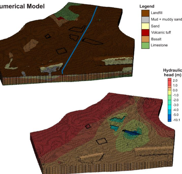
Figure 4. Dimensions, underground structures and characteristics of a numerical model developed for the Alcântara valley (Lisbon)
