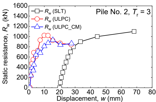
Figure 7. Comparison of load-displacement curves from SLT, RLTs with ULPC and ULPC_CM (Pile No. 2).
