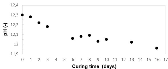
Figure 6. pH values - slurry of soil+2%FA+2%QL.
