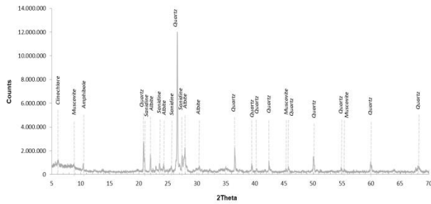
Figure 1. X-Ray diffraction spectrum of the soil.
