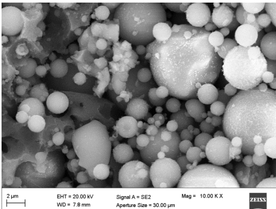
Figure 2. SEM images of the FA (Magnification: 2000x).
