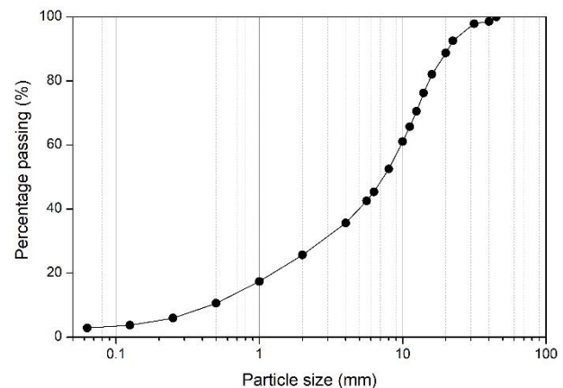
Figure 2. Particle size distribution of IBA.
