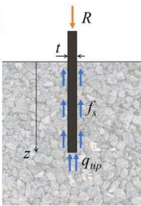
Figure 1. Plate penetration problem and calculation based on bearing capacity.
