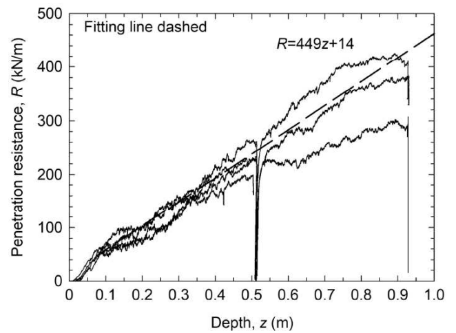
Figure 5. Penetration resistance of 80-mm-thick skirt in 1-3 in. gravel.
