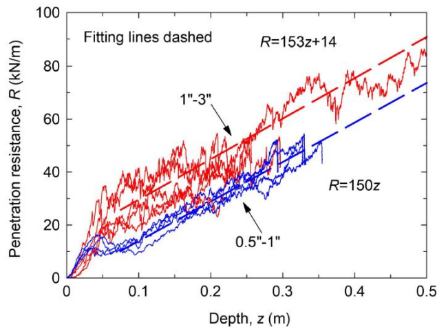
Figure 4. Penetration resistance of 15-mm-thick skirt in both gravels.
