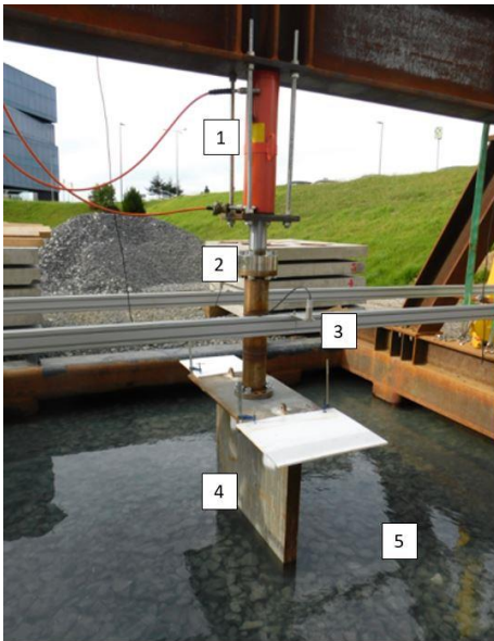
Figure 3. Test set-up. 1-hydraulic jack; 2-load cell; 3-displacement sensor; 4-steel plate; 5-eclogite gravel.
