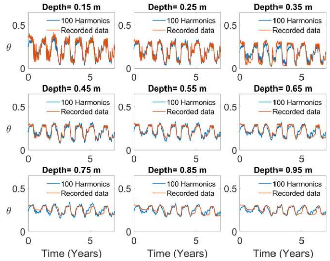
Figure 5. \theta prediction considering 100 harmonics.
