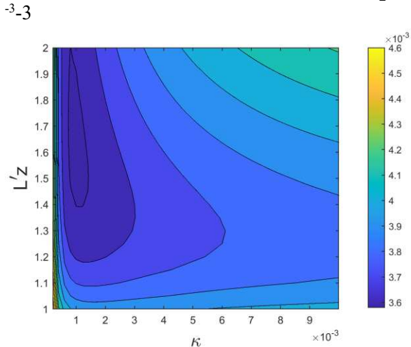
Figure 4. MSE as a function of \kappa and L'_z .
