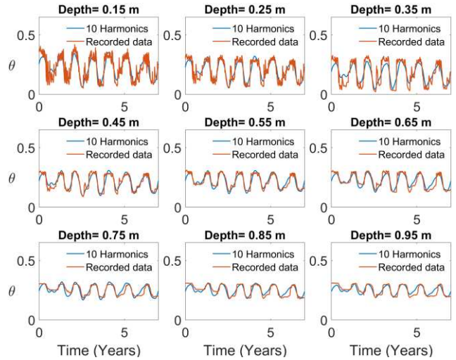
Figure 6. \theta prediction considering 10 harmonics.
