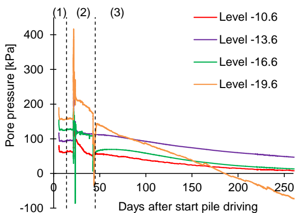
Figure 11. Pore pressure measurements over the entire period (day 250 = 25th of September 2015). Stage (1), (2) and (3) = before, during and after pile driving near piezometers.
