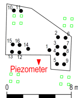
Figure 5. Piles driven at day 21. Numbers refer to the sequence of driving.
