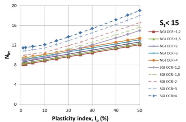
Figure 11 A comparison between the N_{kt} factors suggested by Karlsrud et al. (2005) and SGI (2007) for the clays having S_t < 15 .
