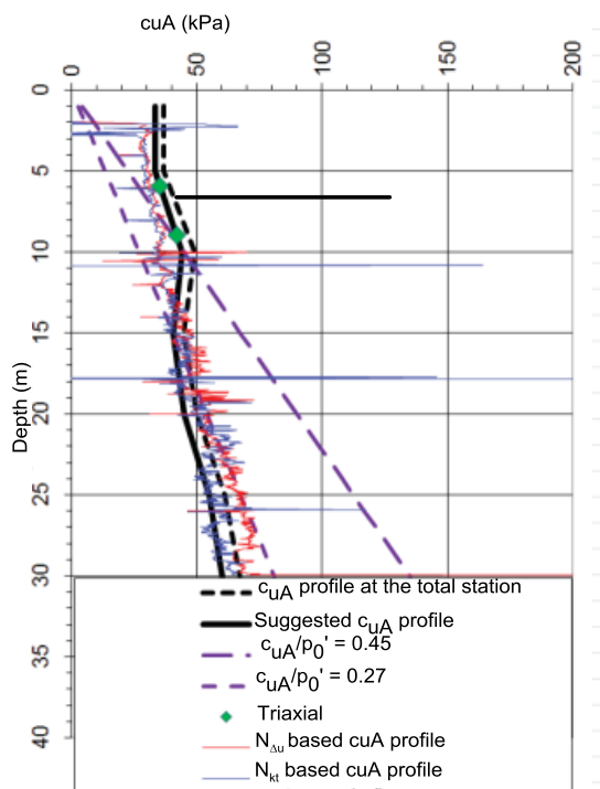
Figure 15 Representative c_{uA} profile at a location where insufficient information is available.
