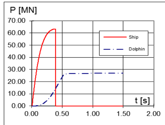
Figure 15 Force in ship’s bow and dolphin
