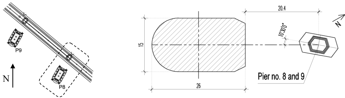
Figure 4 Placement of dolphin in relationship to the pier, overview (left) and detail (right)
