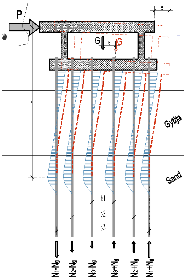
Figure 9 Static system
