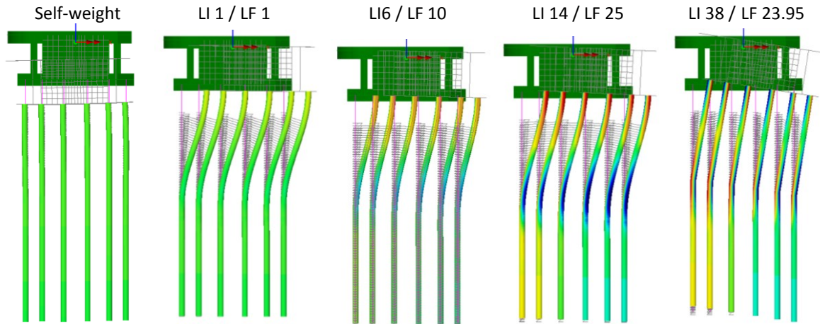
Figure 11 Successive deformed configurations of the dolphin (LI – load increment, LF – load factor)
