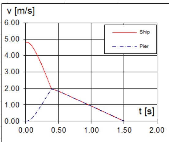
Figure 14 Speed of ship and dolphin over the time
