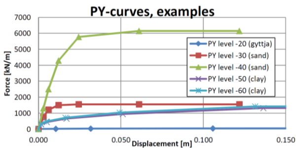
Figure 7 Examples of PY-curves used for piles at pier 9.
