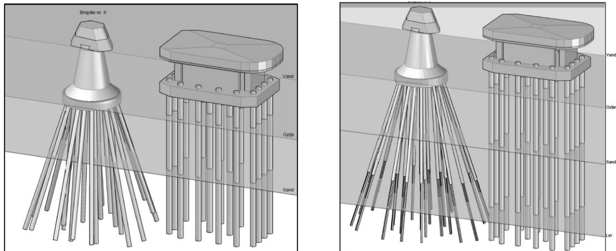
Figure 6 Isometric view of the dolphin and pier 8 (left) and 9(right)
