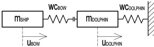
Figure 13 Simplified model for collision analysis
