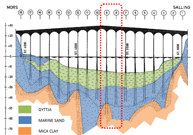
Figure 5 Overview of geotechnical layers which govern the foundation of the bridge
