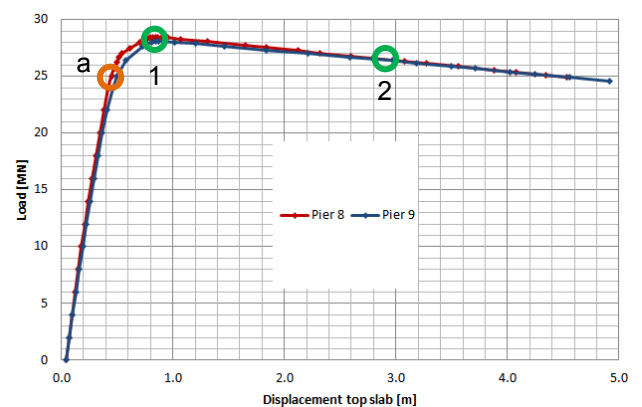
Figure 10 Load-displacement curve of the dolphin 8(red) and 9 (blue)
