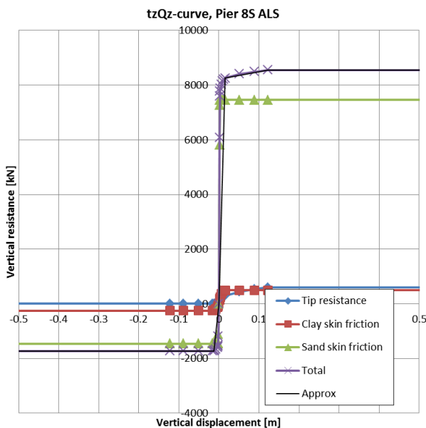
Figure 8 Components of the pile vertical capacity at piers 8 and 9 – TZ curves
