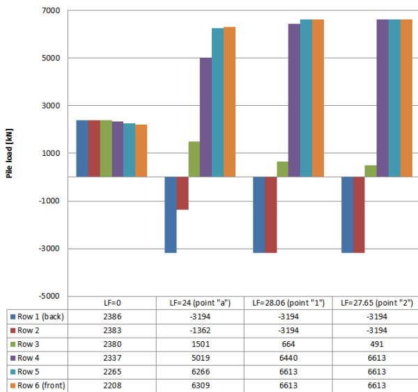
Figure 12 Overview of the development of normal forces in the piles compared to the load factor (each coloured bar corresponds to one row of piles and positive values represent compression)
