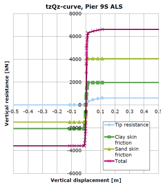
Figure 8 Components of the pile vertical capacity at piers 8 and 9 – TZ curves
