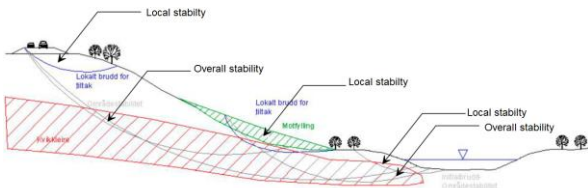
Figure 4 Local and overall stability (NIFS report 72-2012; www.naturfare.no ).
