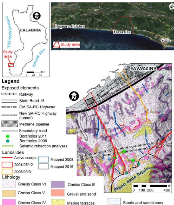
Figure 1. Geographical localization of the study area and weathering grade map of the Favazzina slope
