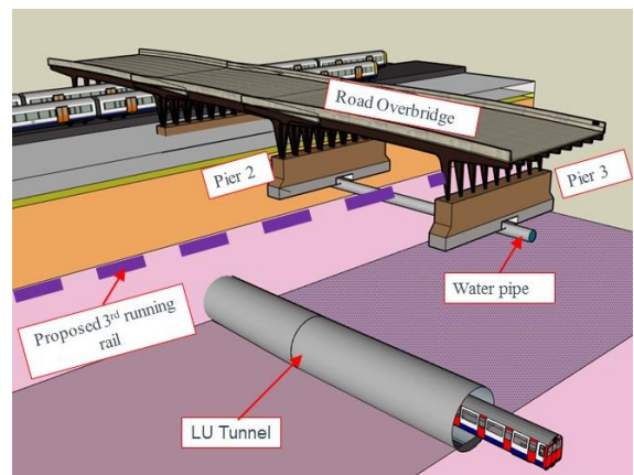
Figure 5. 3D schematic representation of the design constraints at the road overbridge location.
