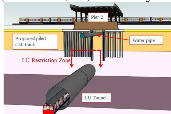
Figure 6. Schematic representation of the proposed solution.
