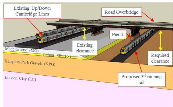
Figure 3. Schematic 3D representation of the clearance.
