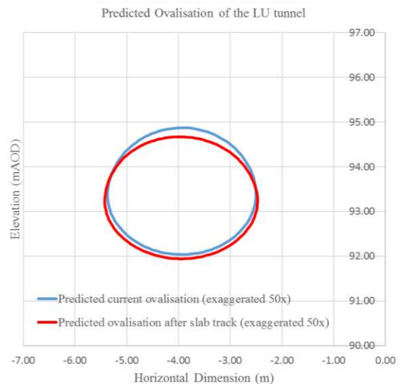
Figure 7. Predicted ovalisation of the LU tunnel.
