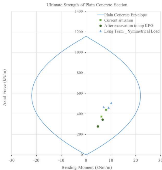
Figure 8. Ultimate moment thrust envelope for the LU tunnel lining against N-M design forces.
