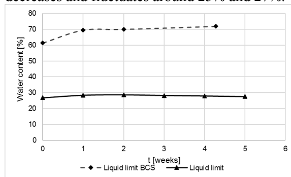
Figure 10: Comparison with literature, liquid limit
