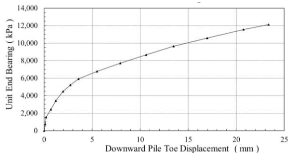
Figure 13 – Mobilised Unit end bearing in Stage 1
