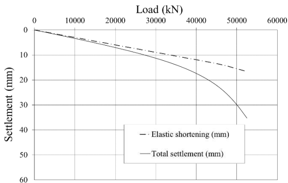
Figure 14 Cemset Pylon Pile head prediction
