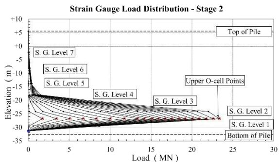
Figure 10 – Strain Gauge load distribution Stage 2 for each loading step
