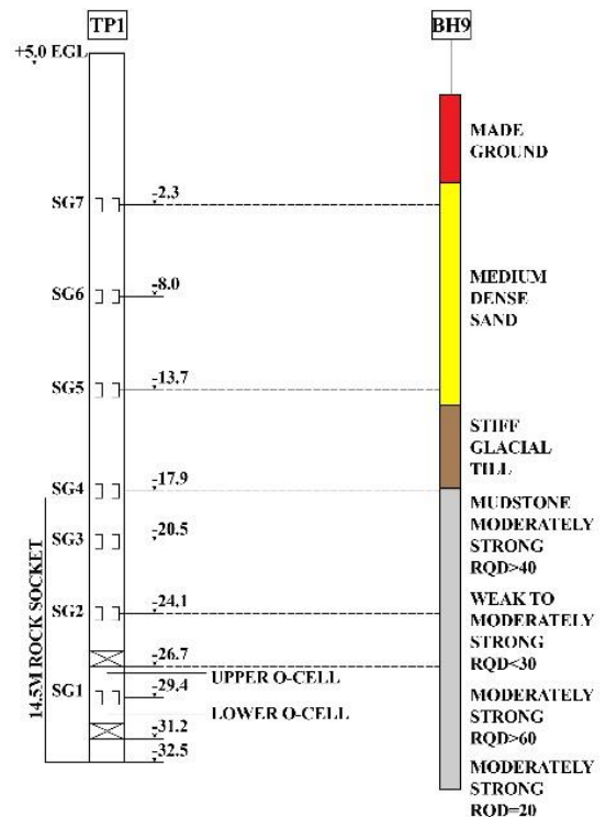
Figure 2. Geology & Instrumentation at Test Pile
