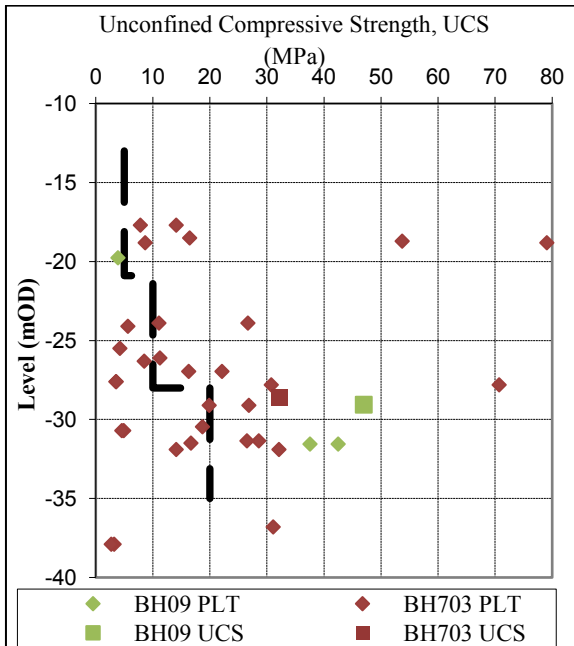
Figure 4 UCS v Level at Preliminary Test Pile
