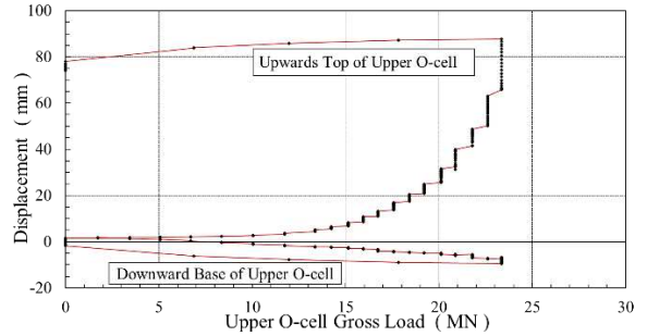
Figure 8 Load displacement of upper O-cell Stage 2
