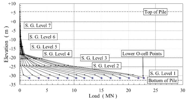
Figure 9 Strain Gauge load distribution Stage 1 for each loading step
