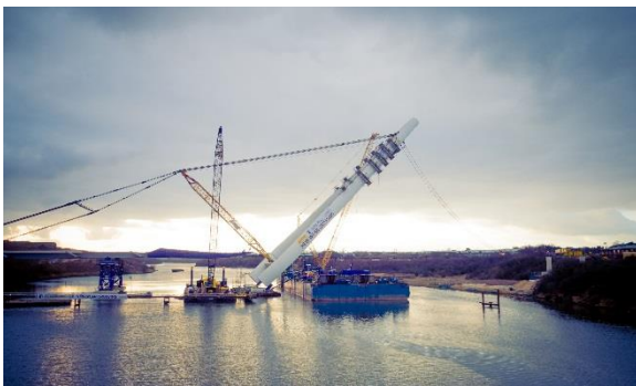
Figure 1. Bridge pylon during erection, February 2017.
