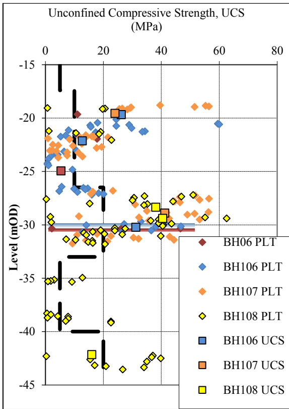
Figure 3. UCS v Level at bridge pylon
