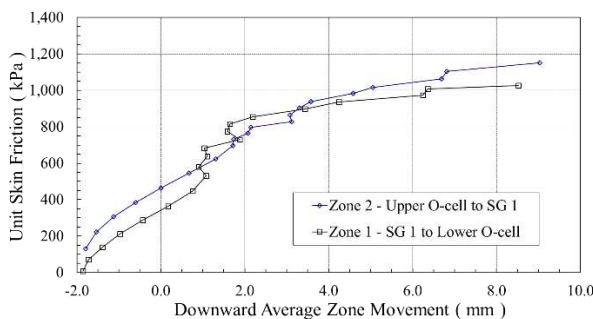
Figure 12 – Mobilised unit skin friction – Stage 2
