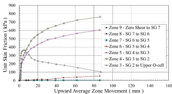
Figure 11 – Mobilised unit skin friction – Stage 2
