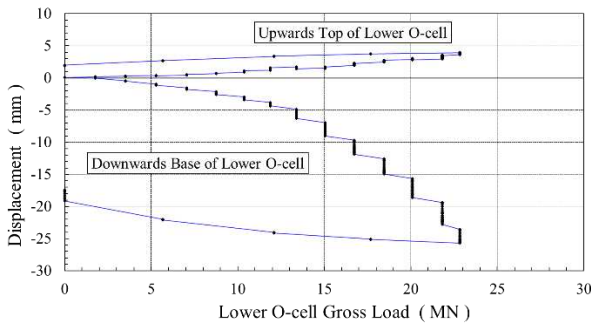
Figure 7- Load displacement of lower O-cell Stage 1
