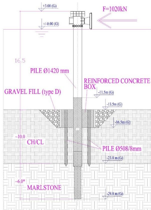
Figure 2. Cross section
