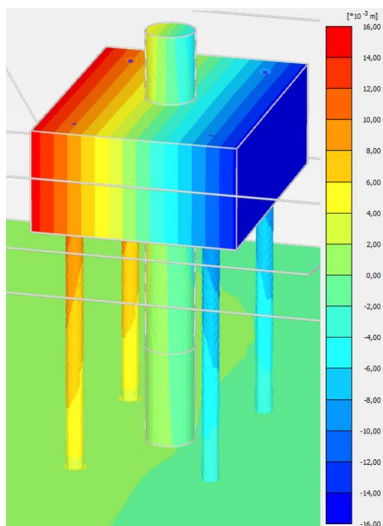
Figure 6. Vertical displacements U_z [m] beneath the seabed - type D ( U_z \approx \pm 1.6\text{cm} )
