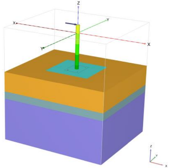
Figure 3. Numerical model (Plaxis 3D)
