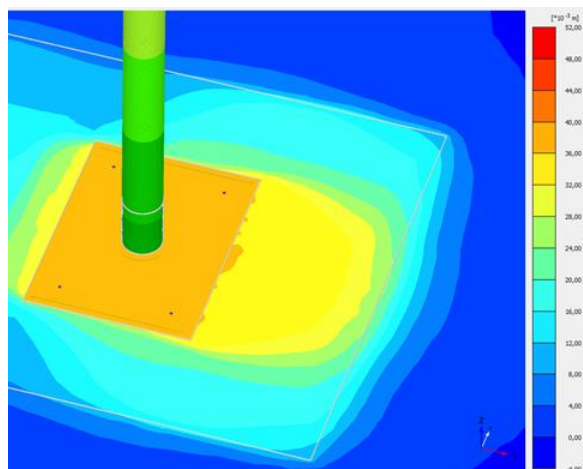
Figure 5. Horizontal displacements at the seabed ( -13.5\text{m} ) - type D ( U_{x\text{max}} \approx 5\text{cm} )
