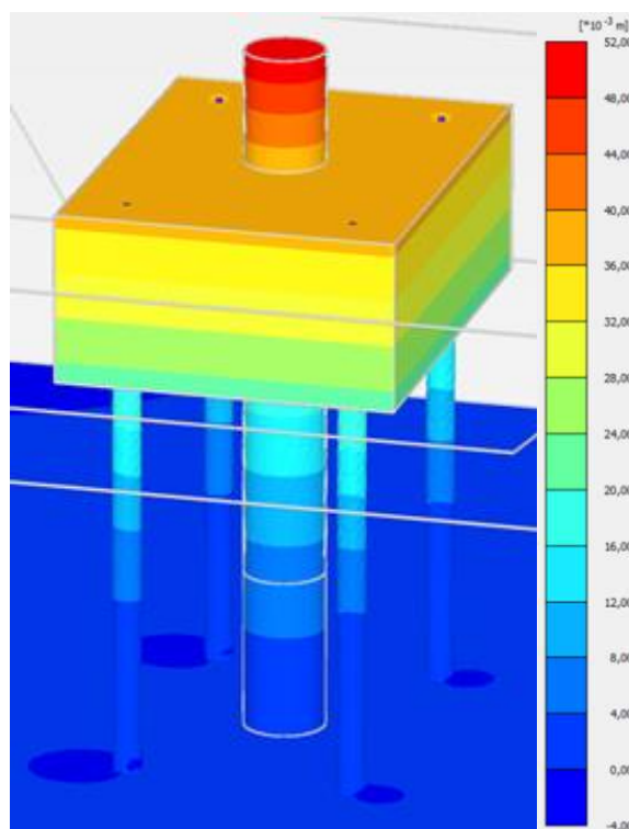
Figure 4. Horizontal displacements beneath the seabed U_x [m] - type D
