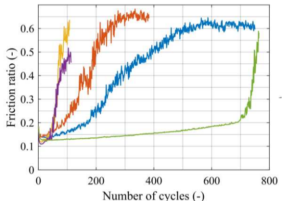
Figure 5. Characteristic friction ratio for 10mm displacement tests vs. number of cycles
