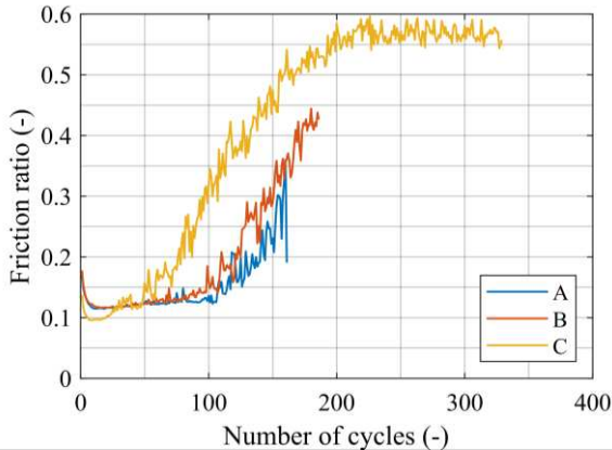
Figure 6. Tests stopped at 0.3 (A) and 0.4 (B) friction ratios and one previous test (C)
