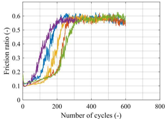
Figure 4. Characteristic friction ratio for 6mm displacement tests vs. number of cycles
