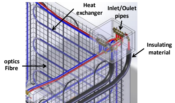
Figure 2. Position of heat exchanger pipes
