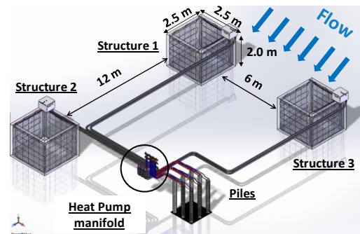
Figure 3. Disposition of energy geostructures
