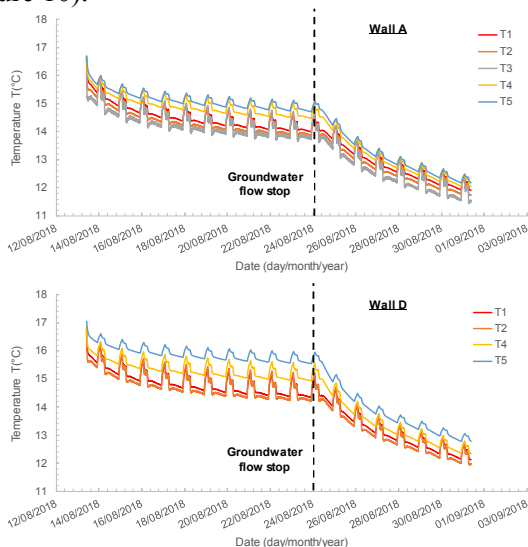
Figure 10. Concrete temperature variation for wall A and D of structure 1
