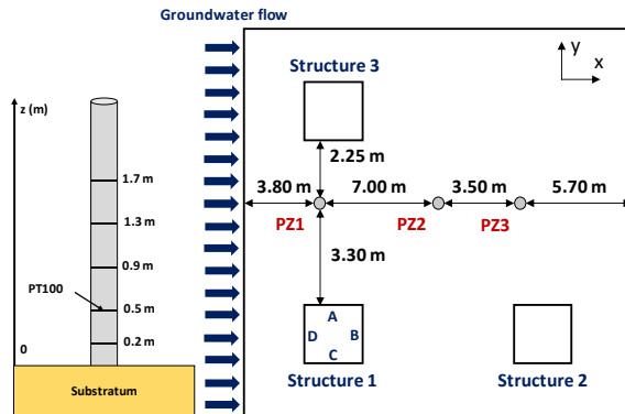
Figure 4. PT100 position on piezometer
