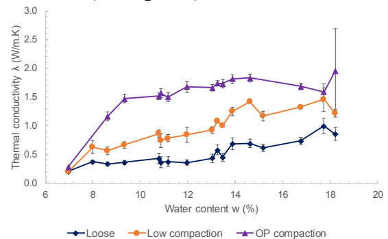
Figure 7. Thermal conductivity at different water content and density
