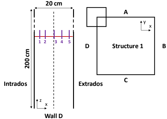
Figure 5. PT100 position in concrete
