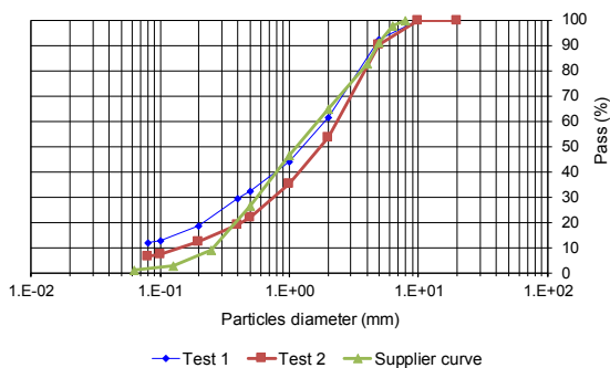
Figure 6. Particle size distribution curve
