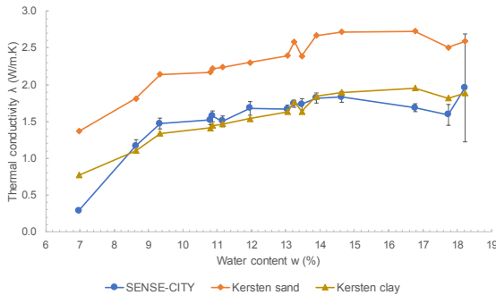
Figure 8. Comparison between Kersten conductivity and measured conductivity
