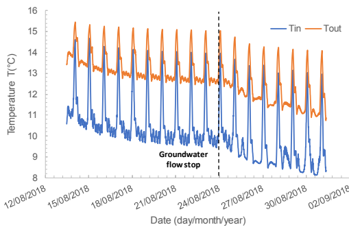
Figure 9. Inlet and outlet fluid temperature variation in structure 1
