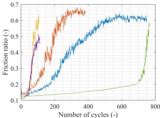
Figure 5. Characteristic friction ratio for 10mm displacement tests vs. number of cycles
