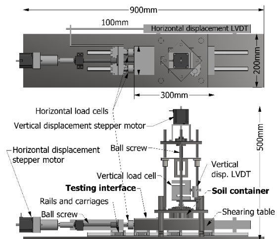
Figure 1. Detailed view of the soil-interface shearing device
