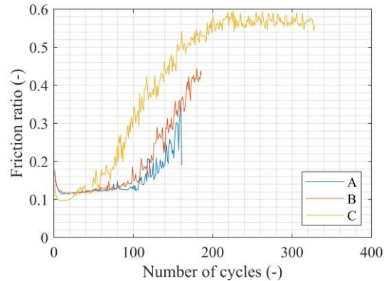
Figure 6. Tests stopped at 0.3 (A) and 0.4 (B) friction ratios and one previous test (C)
