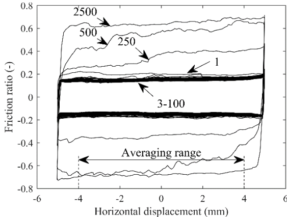
Figure 2. Typical cyclic response of friction ratio vs. horizontal displacement with cycle numbers labelled
