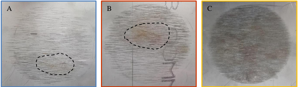
Figure 7. Damage of the steel plate at (A) 0.3 friction ratio, (B) 0.4 friction ratio and (C) full damage
