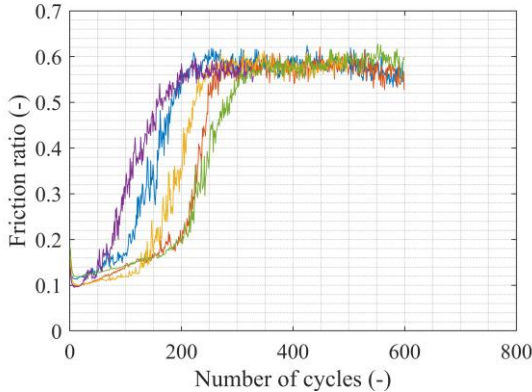
Figure 4. Characteristic friction ratio for 6mm displacement tests vs. number of cycles
