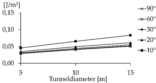
Figure 6. Linear relation between the specific heat work and the flow geometry
