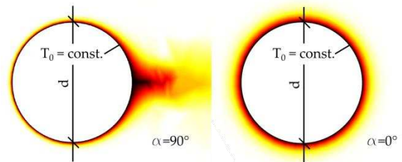
Figure 3. Temperature corona around a thermally activated tunnel for a temperatur range of 0°C (dark) to 10°C (light)
