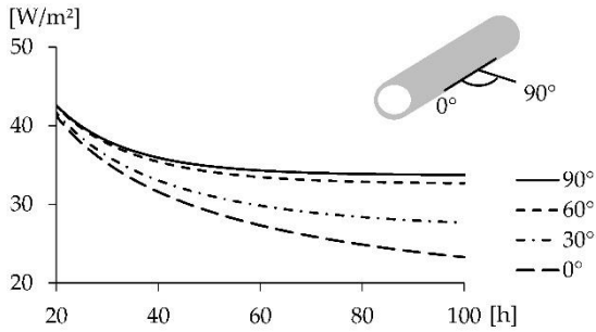
Figure 4. Time-dependent behaviour of the extractable heat flux density under different ground water flow directions
