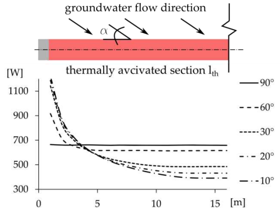
Figure 5. Integral heat flux for each meter of tunnel along the tunnel axis
