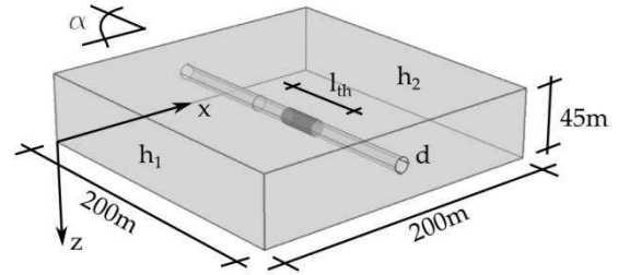
Figure 2. Isometric view of the calculation model to investigate an oblique ground water flow onto a tunnel geothermal plant
