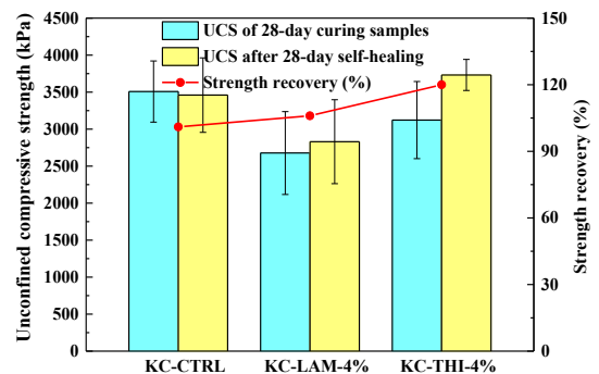
Figure 9 Unconfined compressive strength recovery after 28 days of self-healing
