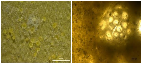
Figure 6 Optical microscope images of LAM (left) and THI (right) microcapsules in fresh soil mix wall materials
