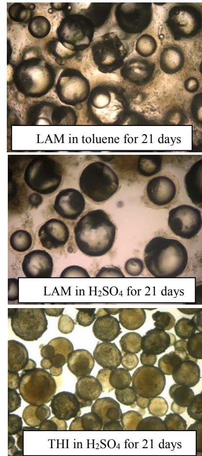
Figure 4 Optical microscope images of microcapsules in different chemical environments
