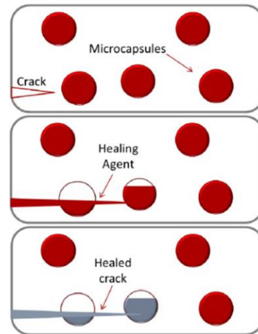
Figure 1. The concept of autonomic microcapsule-based self-healing (Souza, 2017)
