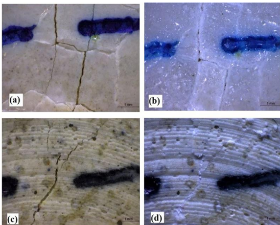
Figure 8 Typical stereoscope images of crack mouth taken on the day of cracking (left) and after 28 days of self-healing (right) for (a,b) LAM-containing sample and (c,d) THI-containing sample
