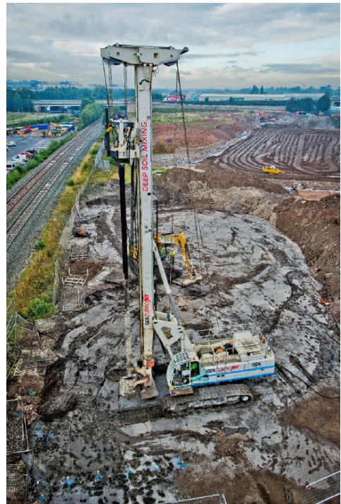
Figure 1. Turbojet system for deep soil mixing (courtesy of Ground Developments Ltd)
