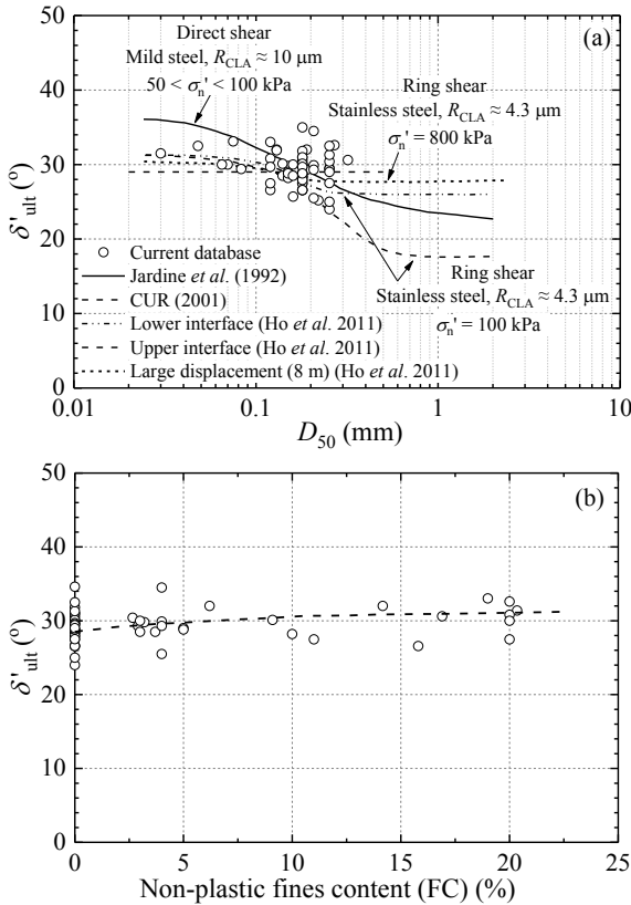
Figure 3. (a) Comparison of \delta'_{ult} against D_{50} with published trends; (b) Correlation between \delta'_{ult} and fines content (FC)
