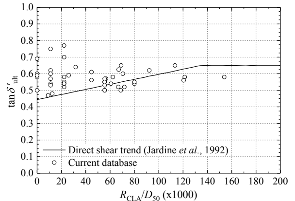
Figure 5. Correlation between \tan(\delta'_{ult}) and pre-test normalised roughness R_{CLA}/D_{50}
