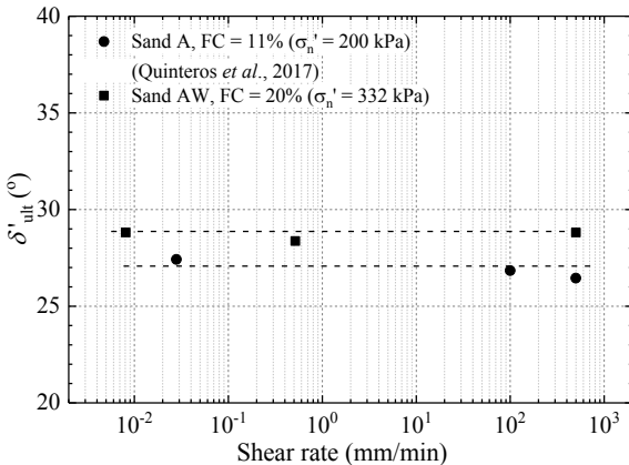
Figure 7. Shear rate effects: \delta'_{ult} against shear rates
