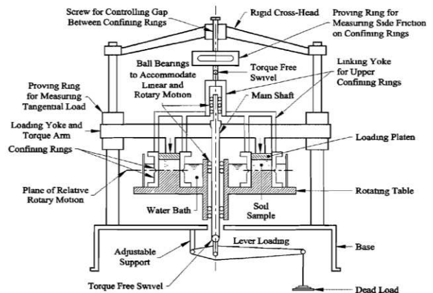
Figure 1. Soil interface configuration of Bishop ring shear apparatus (Bishop et al. , 1971, Ramsey et al. , 1998)
