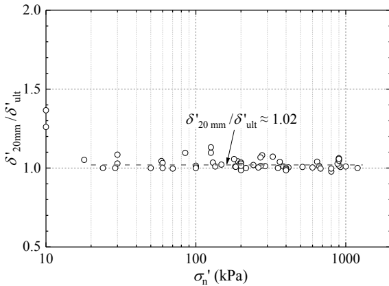
Figure 6. Correlation between \delta'_{20mm}/\delta'_{ult} against \sigma'_n
