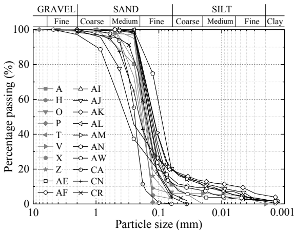
Figure 2. Ranges of grain size distribution of the soils
