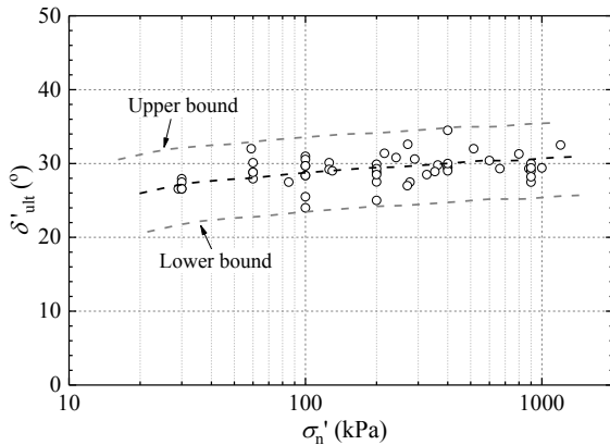
Figure 4. Correlation between \delta'_{ult} and \sigma'_n
