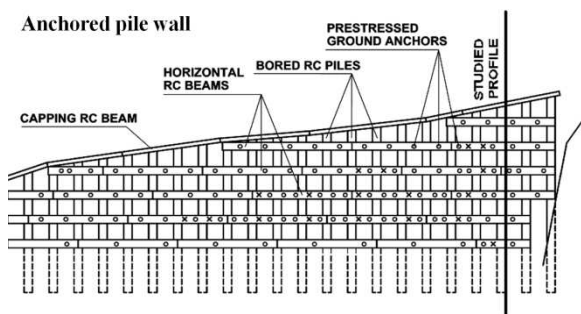
Figure 2. View of the retaining structure
