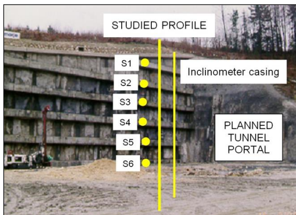
Figure 3. Monitoring system at the studied profile
