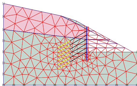
Figure 4. Geometrical model at the studied profile
