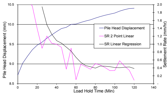
Figure 2. Settlement rates, calculated by equation 1 and equation 2.
