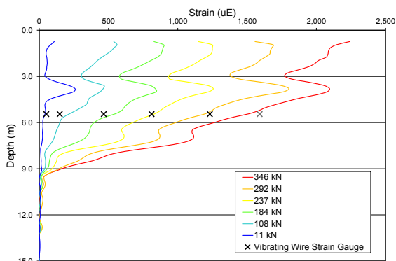
Figure 4. DFOS and VWSG results for a tension test on a micro pile.
