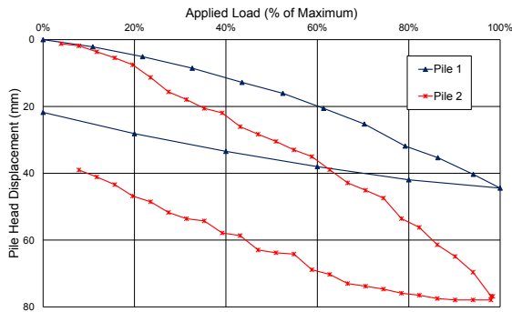
Figure 3. Pile head displacements from load test data presented in Table 1.
