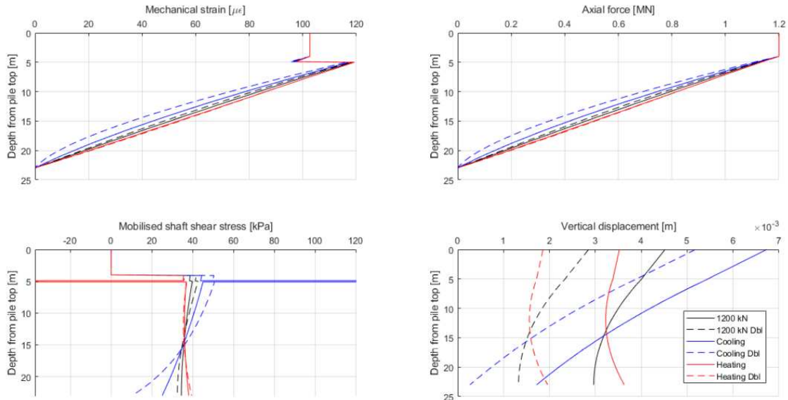
Figure 5. Comparison between Doubled soil stiffness (dashed lines) and unmodified soil stiffness (continuous lines) for mechanical loading case (black), cooling phase (blue) and heating phase (red)
