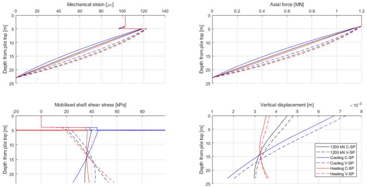
Figure 3. Comparison between Constant Soil Parameters (continuous lines) and Variable Soil Parameters (dashed lines) with depth for mechanical loading case (black), cooling phase (blue) and heating phase (red)
