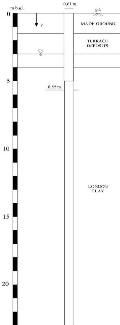
Figure 2. Sketch of the Lambeth College test energy pile and soil stratigraphy
