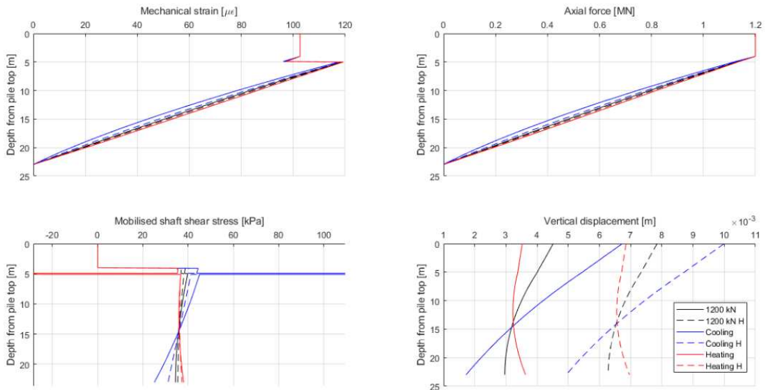
Figure 6. Comparison between Halved soil stiffness (dashed lines) and unmodified soil stiffness (continuous lines) for mechanical loading case (black), cooling phase (blue) and heating phase (red)
