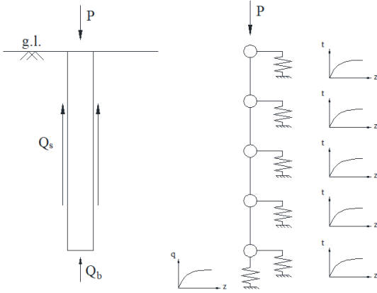
Figure 1. Discretisation of the axially-loaded pile into two-noded beam elements within the load-transfer FE model
