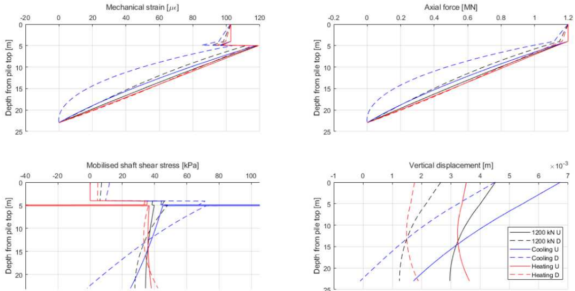
Figure 4. Comparison between Undrained (continuous line) and Drained (dashed lines) conditions for mechanical loading case (black), cooling phase (blue) and heating phase (red)
