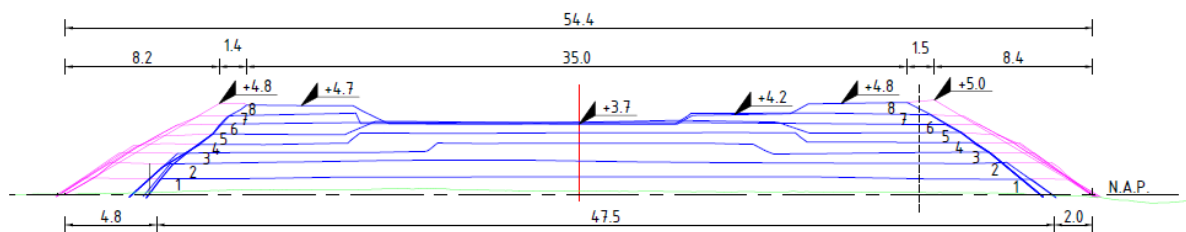
Figure 4: Layered construction of test levees
