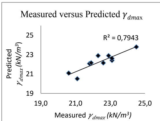
Figure 3: Predicted and measured \gamma_{dmax} for validation
