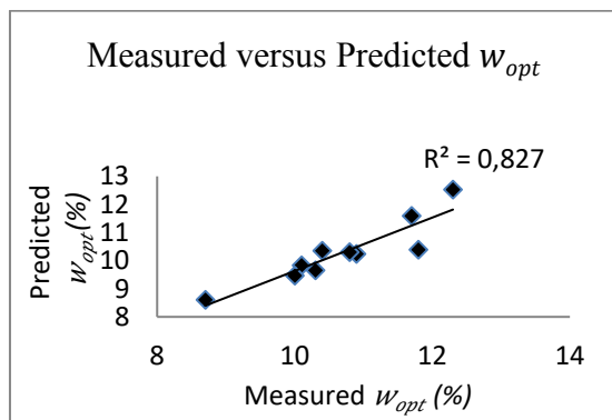
Figure 4: Predicted and measured w_{opt} for validation
