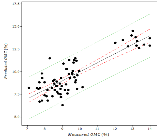
Figure 2: Comparison of predicted and measured w_{opt}
