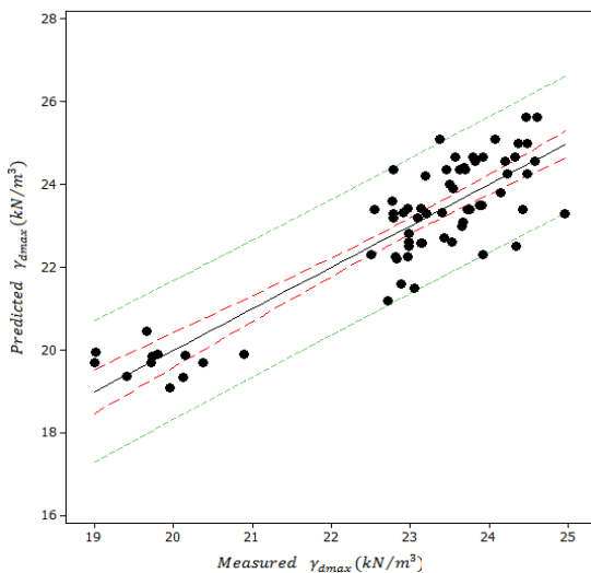
Figure 1: Comparison of predicted and measured \gamma_{dmax}
