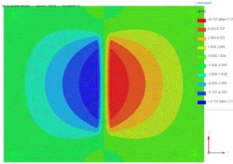
Figure 12: Displacement of the soil in the numerical model with Mohr Coulomb law in Cesar LCPC
