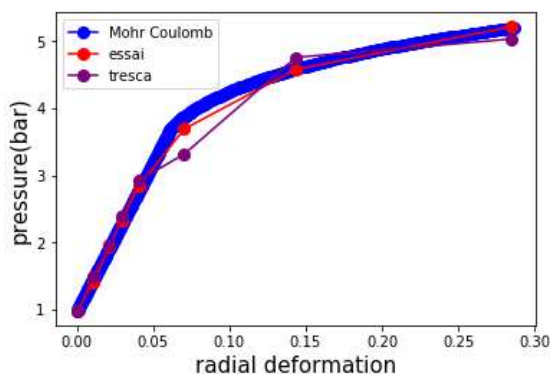
Figure 10: Analytical simulation of a real in situ test with Mohr Coulomb and Tresca models (Python software)
