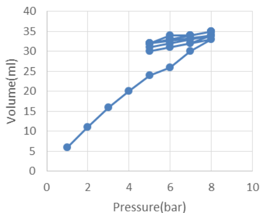
Figure 16: Pressure volume curve
