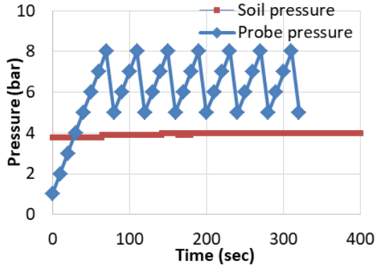
Figure 17: Reaction of the soil sample to the pressuremeter test
