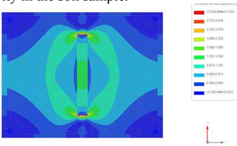
Figure 13: Deviatoric stress in the numerical model
