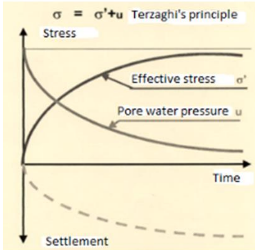
Figure 1: Terzaghi's principle
