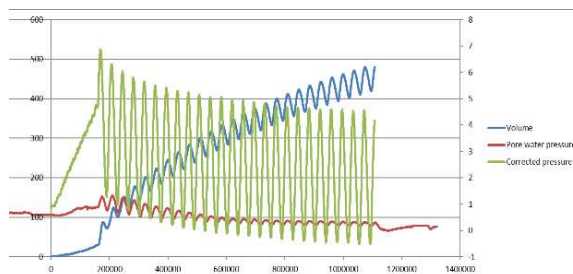
Figure 5: Cyclic tests with measurement of pore water pressure
