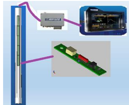
Figure 3: Set of equipment for measurement and reading of the pore water pressure
