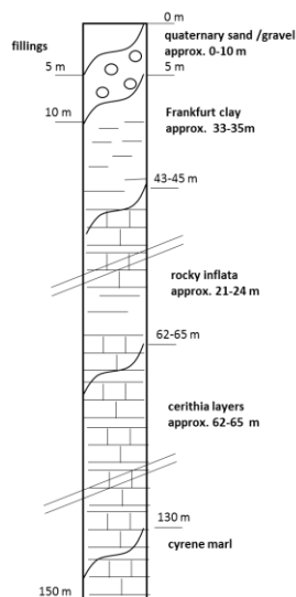
Figure 2. Schematic soil model
