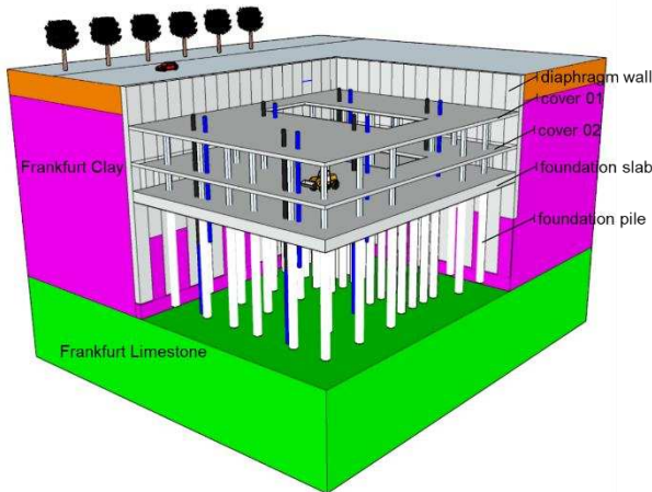
Figure 3. Top-down technique
