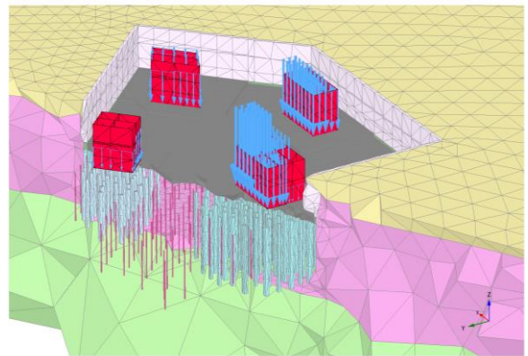
Figure 5. Numerical model - Constructive elements
