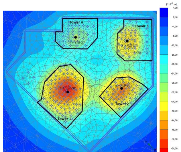
Figure 6. layout – Settlements of the towers
