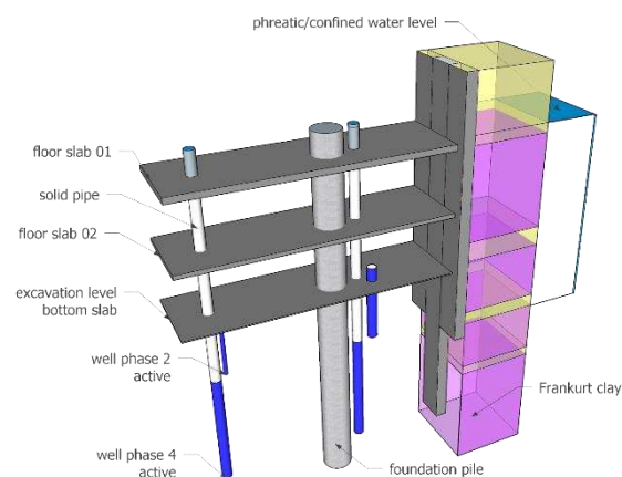
Figure 10. Dewatering phase 4
