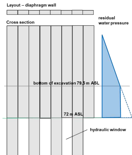
Figure 7. Residual water pressure
