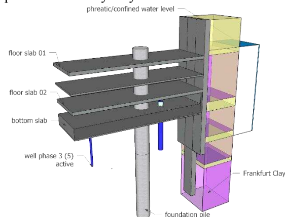
Figure 11. Dewatering phase 5
