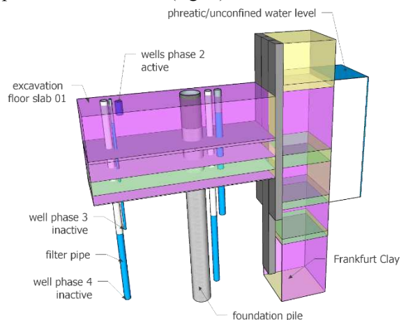
Figure 8. Dewatering phase 2
