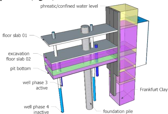
Figure 9. Dewatering phase 3
