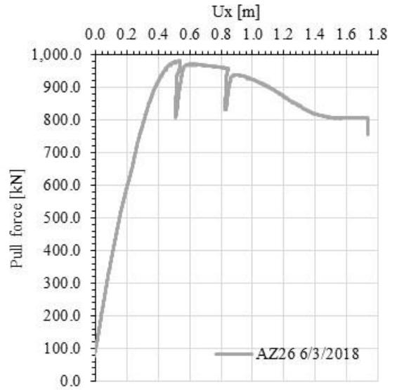
Figure 12. Force-displacement diagram AZ26 AZ26 2018-03-06 12:34:00
