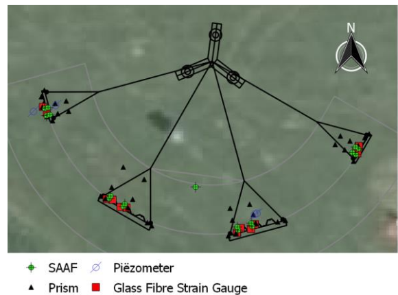
Figure 3. Top view POT site with monitoring instrumentation
