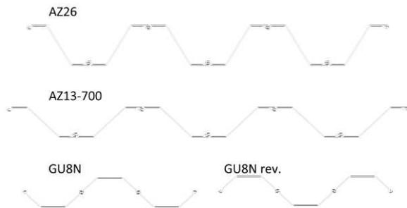
Figure 2. Sheet pile profiles
