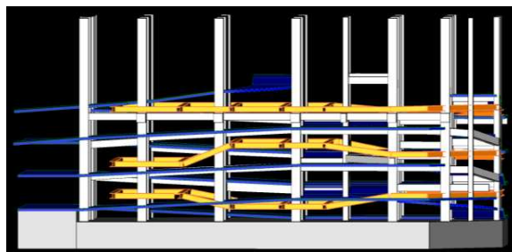
Figure 2. BIM model of strutting arrangement (Tanaka et al., 2017)
