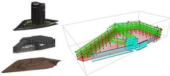
Figure 3. 3D Architecture and the retaining BIM model (Gondar et al., 2018)
