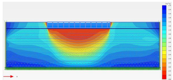
Figure 7. Settlements due to dewatering
