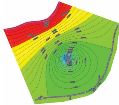
Figure 6. Hydro-dynamic spectrum with the influence of dewatering
