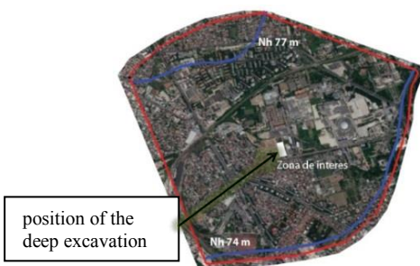
Figure 5. Hydrogeological model and boundary conditions
