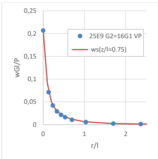
Figure 4. Soil settlement z=0.75l , points - pile settlement. G_2=16G_1 .
