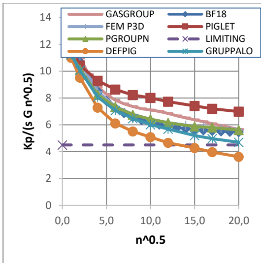
Figure 8. Comparison of pile group settlement by IFM with FEM and published results ( s=2.5d )
