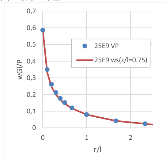
Figure 3. Soil settlement z=0.75l , points - pile settlement. Uniform soil.
