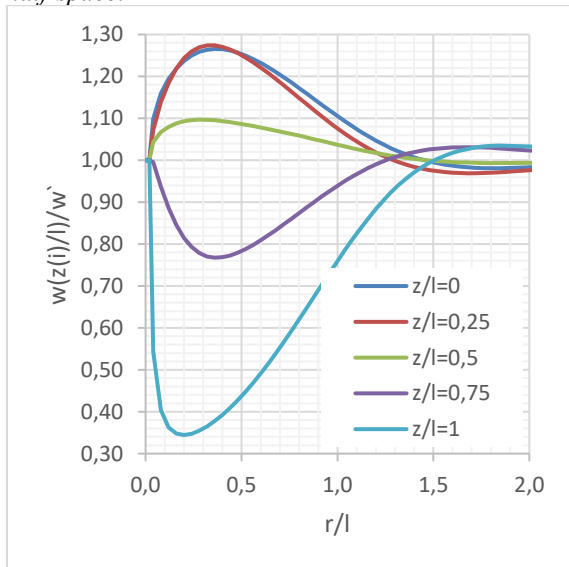
Figure 1. Settlement of soil with distance for given depths normalized by average soil settlement. Two-layer soil, bottom layer 16 times stiffer.
