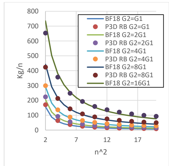
Figure 7. Comparison of IFM result with FEM.
