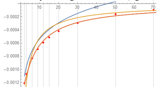
Figure 10. Additional settlement of soil due to interaction of piles of 40 and 50m. Points are FEM results. Red line - proposed approach.
