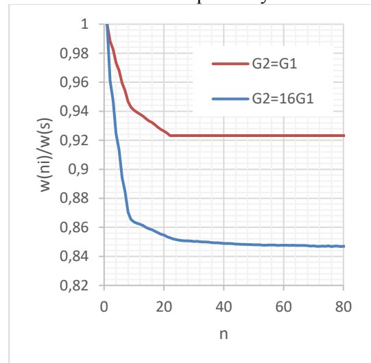
Figure 6. Reduction of single pile settlement in presence of unloaded piles.
