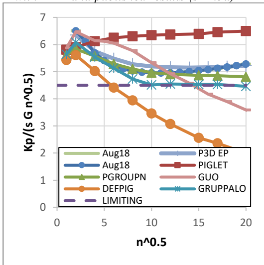
Figure 9. Comparison of pile group settlement by IFM with FEM and published results ( s=5d )
