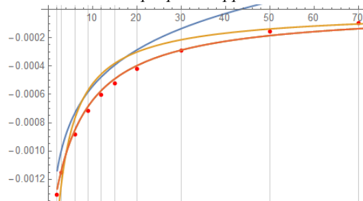
Figure 11. Additional settlement of soil due to interaction of piles of 10 and 60m. Points are FEM results. Red line - proposed approach.
