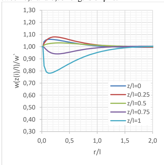
Figure 1. Settlement of soil with distance for given depths normalized by average soil settlement. Uniform half-space.
