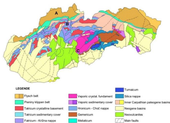
Figure 1. Schematic geological map of Slovakia. A – locality Kycerka, B – locality Korbelka and Cebrat, C – locality Krivan
