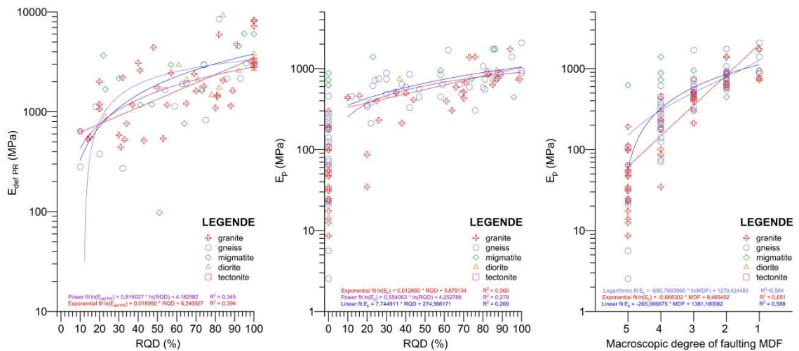
Figure 6. The relation between derived deformation modulus E_{def PR} and RQD from dilatometer tests (left) for Paleozoic crystalline and metamorphic, relation between pressuremeter modulus E_p and RQD (middle) and relation of macroscopic degree of faulting and E_p (right).
