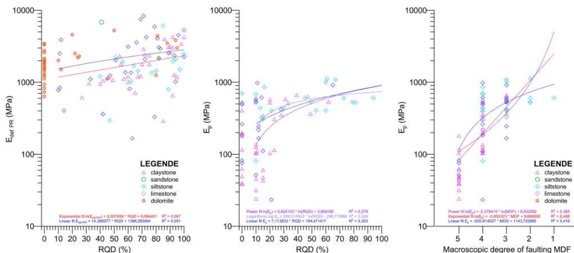
Figure 4. The relation between derived deformation modulus E_{defPR} and RQD from dilatometer tests (left) for Mesozoic rocks, relation between pressuremeter modulus E_p and RQD (middle) and relation of macroscopic degree of faulting and E_p (right).
