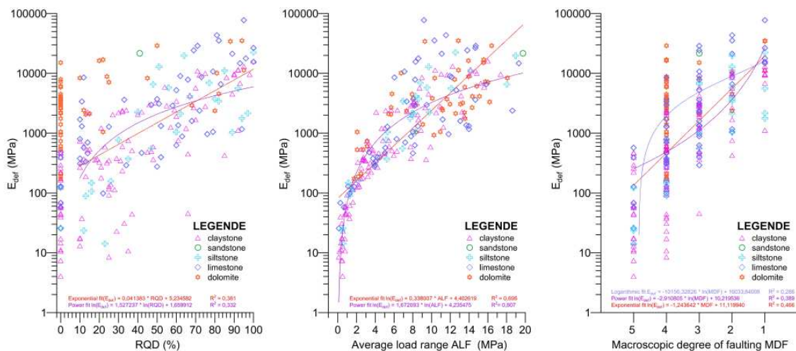
Figure 3. Results of dilatometer tests from Mesozoic sedimentary and carbonate rocks. Relation between deformation modulus E_{def} and RQD (left), average load range (middle) or macroscopic degree of faulting (right).
