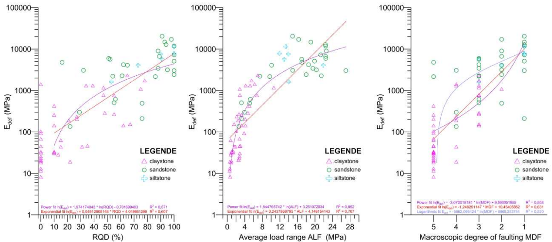
Figure 2. Results of dilatometer tests from flysch rocks. Relation between deformation modulus E_{def} and RQD (left), average load range (middle) or macroscopic degree of faulting (right).
