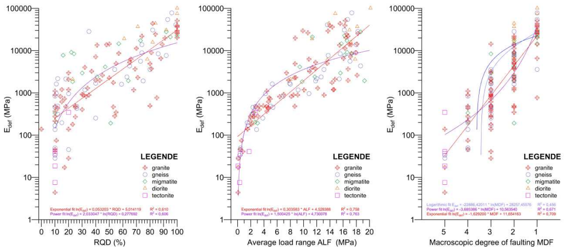
Figure 5. Results of dilatometer tests from Paleozoic crystalline and metamorphic rocks. Relation between deformation modulus E_{def} and RQD (left), average load range (middle) or macroscopic degree of faulting (right).
