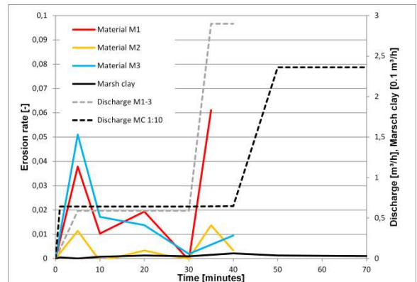
Figure 3. Erosion rates ( V_w/V_s ) from laboratory flume tests
