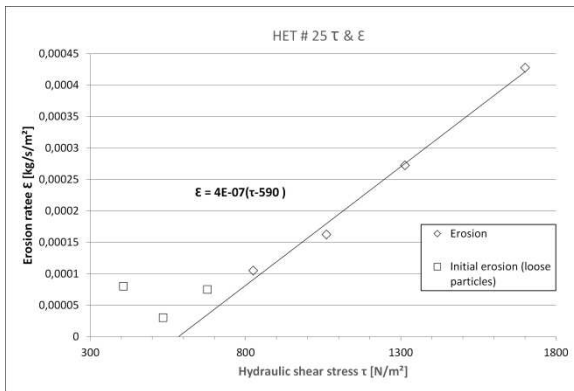
Figure 8. HET results -#25, erosion rate, initiation of erosion
