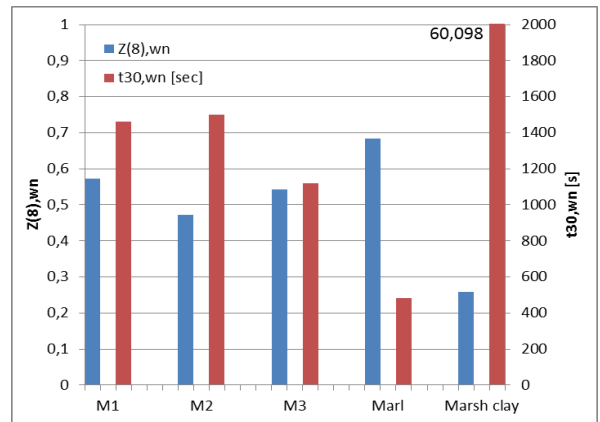
Figure 5. Disintegration numbers z(8) and times t_{30} for initial / natural water content
