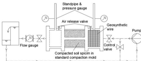
Figure 1. Schematic of disintegration test
