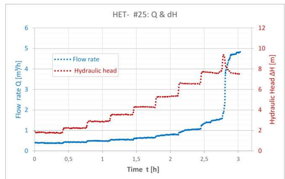
Figure 7. HET results -#25 with 9 different pressure steps, collapse at \Delta H \approx 9\text{ m}
