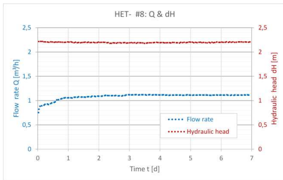
Figure 6. HET results R3 #8; 7 days of continuous high load and stagnating flow rate
