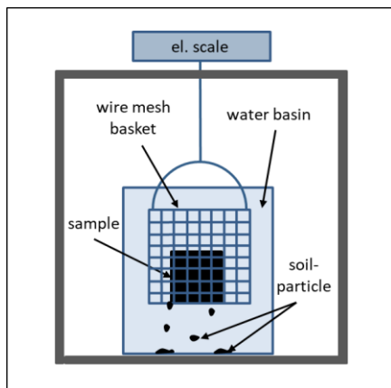
Figure 1. Schematic of disintegration test
