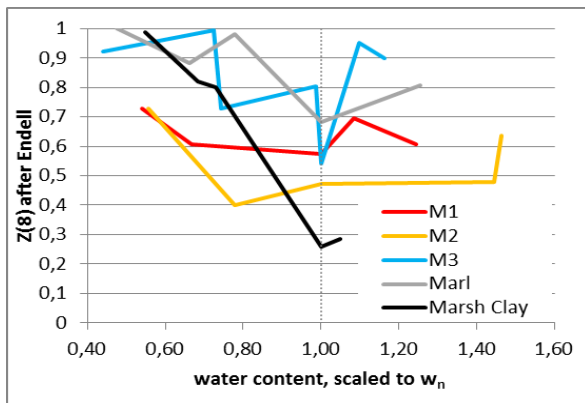
Figure 4. Disintegration numbers vs. normalised water content – justification for the use of w_n
