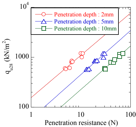
Figure 6. Relationships between penetration resistance and unconfined compressive strength
