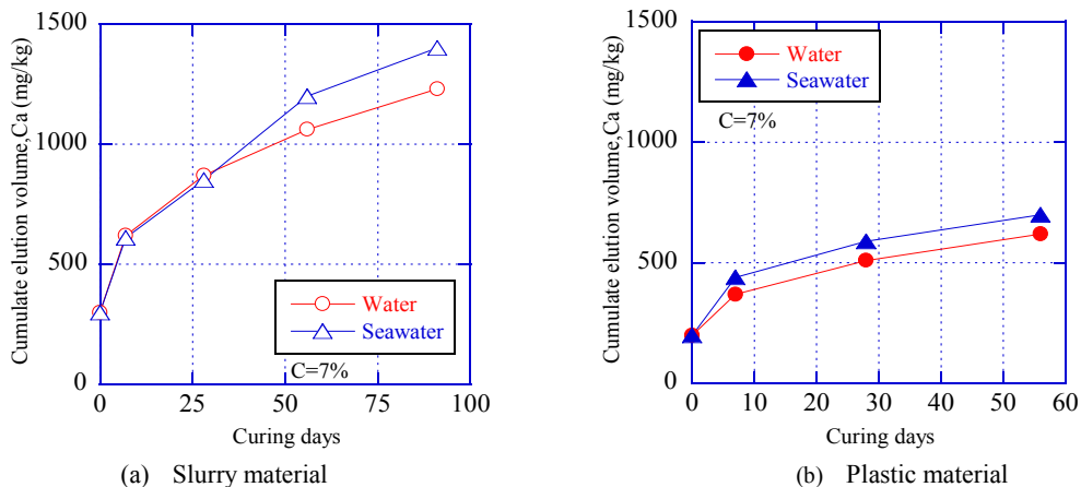
Figure 5. The correlation curing days and the cumulative calcium elution amount (C=7%)
