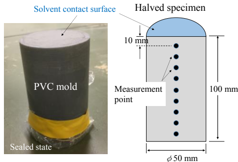
Figure 2. Measurement position of needle pen-
