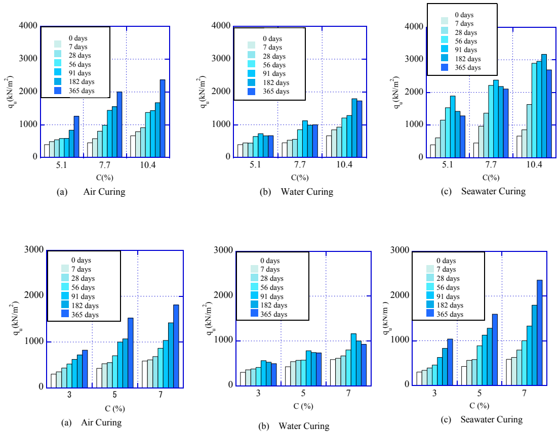
Figure 4. The correlation of UCS ( q_u ) and cement content ( C ) on exposure tests
