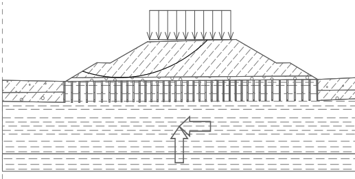
Figure 8. Slope analysis
