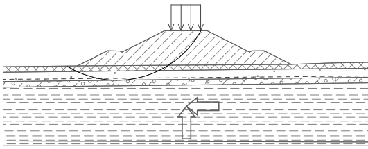
Figure 7. Slope analysis
