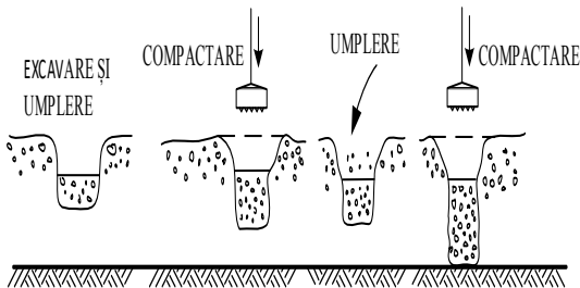
Figure 4. Dynamic compaction
