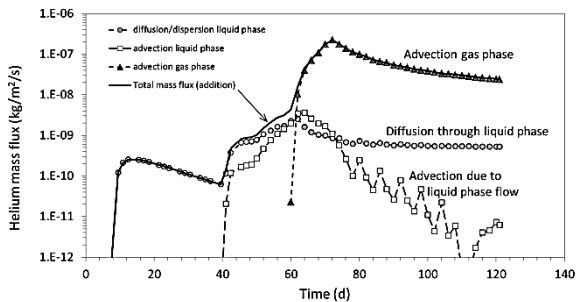
Figure 12. Evolution of the individual components of helium mass flux.
