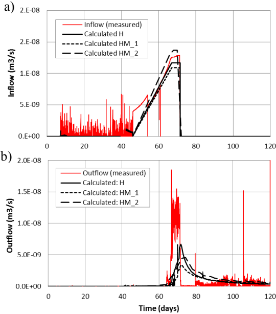
Figure 7. Inflow (a) and outflow (b) evolution results.
