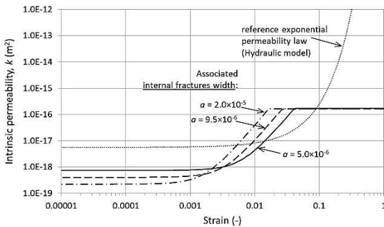
Figure 5. Material intrinsic permeability law: HM_2.
