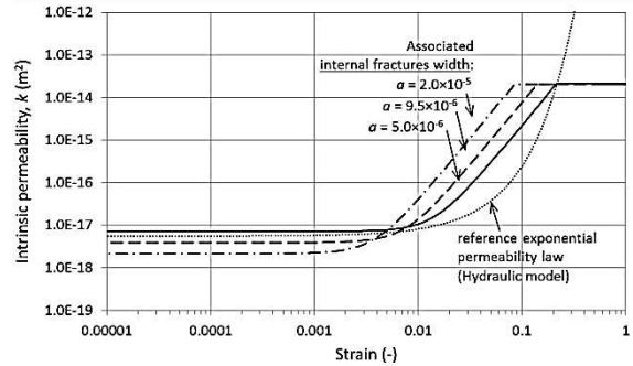
Figure 4. Material intrinsic permeability law: HM_1.
