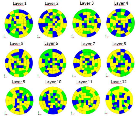
Figure 6. Layer-by-layer random permeability distribution assumed: 2/3 weighting for higher permeability value (yellow: k_0 = 2.2e-19 m 2 ) and 1/6 weighting for the lower values (blue and green, 3.9e-19 m 2 and 7.1e-19 m 2 , respectively).
