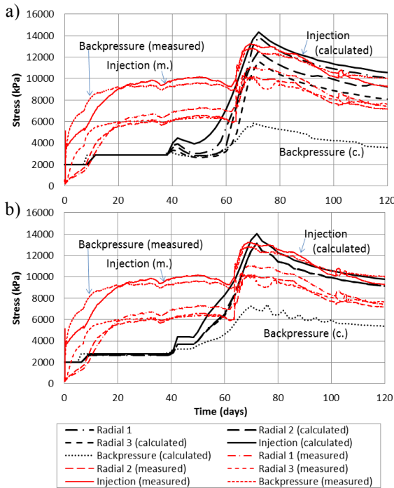
Figure 11. Stress evolution results (hydro-mechanical models): HM_1 (a) and HM_2 (b).
