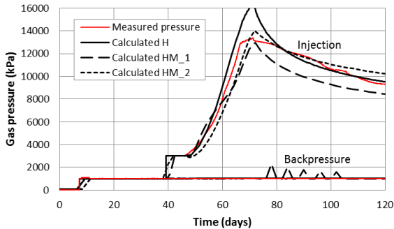
Figure 8. Injection and backpressure evolution results.
