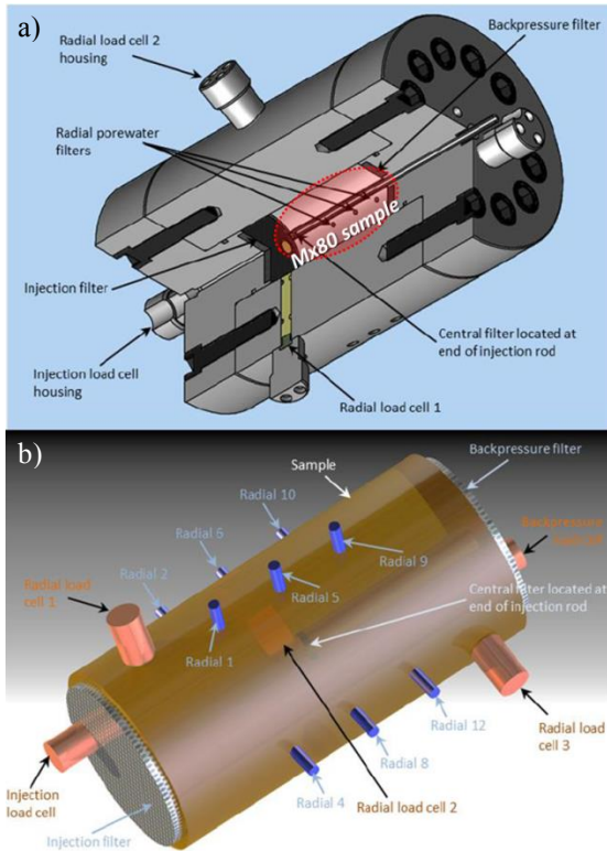
Figure 1. Mx80-D test: main details of pressure vessel (a) and Mx80 sample monitoring locations (b) (modified from Daniels and Harrington 2017).
