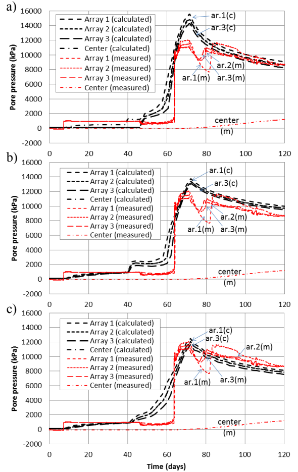
Figure 9. Pore pressure evolution results: Hydraulic model (a), HM_1 (b), and HM_2 (c).
