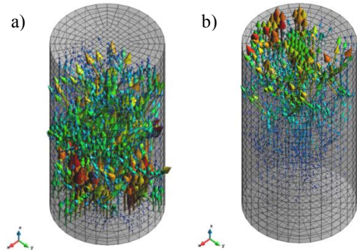
Figure 10. Advective gas flux at day 65 during injection (a) and day 75 during dissipation (b).
