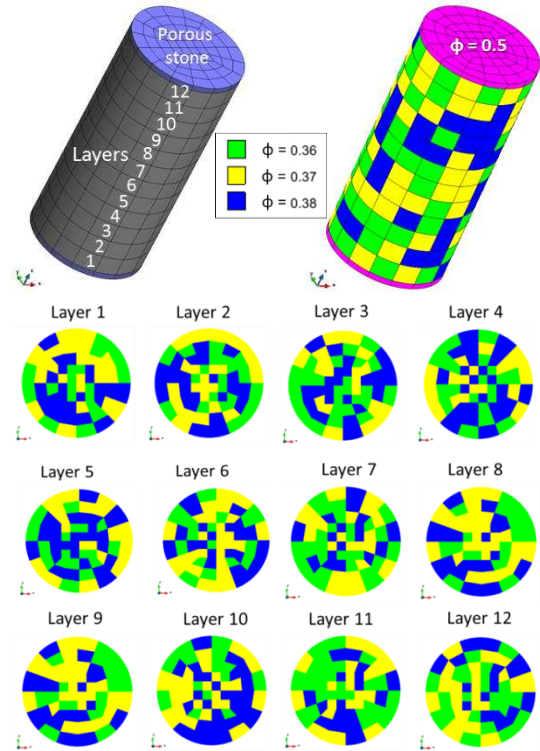
Figure 2. Layer-by-layer random porosity distribution (1/3 weighting each).
