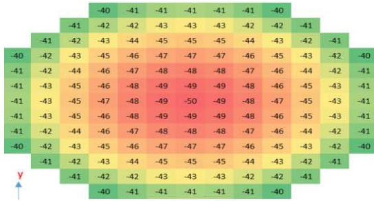
Figure 4. Settlement results for Best Estimate – short term settlements (SB model)
