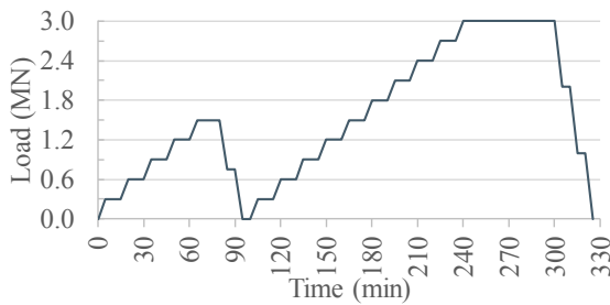
Figure 5. Load steps, digitized cf. (Bartsch, 2018).
