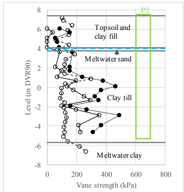
Figure 3. Ground conditions for P2.
