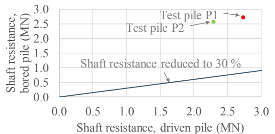
Figure 8. Shaft resistance for bored vs. driven piles.
