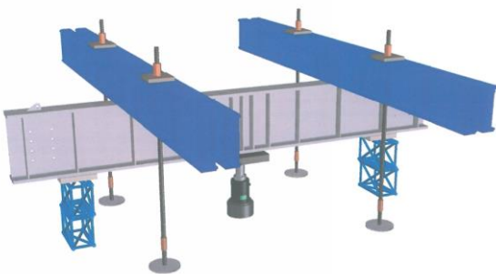
Figure 4. Test set-up for static compression pile load tests (Bartsch, 2018).
