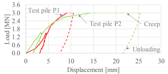
Figure 6. Load-displacement curves for static compression pile load tests on P1 and P2, digitized cf. (Bartsch, 2018).
