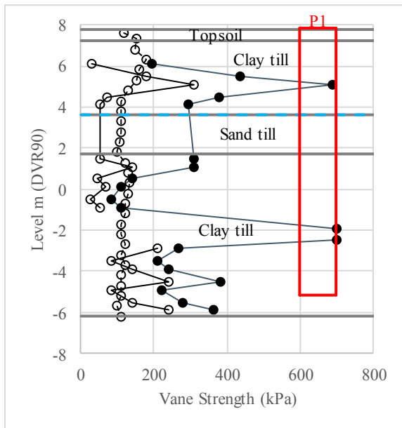
Figure 2. Ground conditions for P1.
