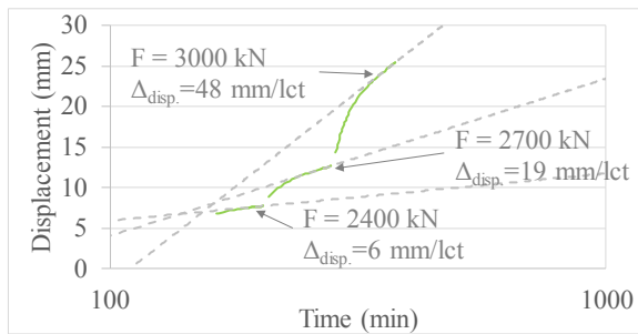
Figure 7. Time-displacement curves for the three last load step of static compression pile load test P2, digitized cf. (Bartsch, 2018).
