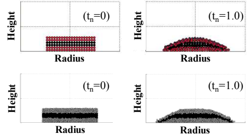
Figure 3. Initial column (at t_n = 0 ) and final deposit profile (at t_n = 1.0 ) for a column with a = 0.55 ; SPH (red/black) and DEM (gray/black)
