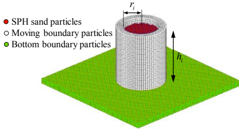
Figure 1. Schematic representation of a 3D SPH cylindrical column
