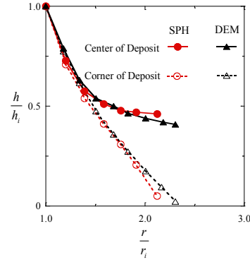
Figure 6. Evolution of normalized height h/h_i for a = 2.0 from SPH and DEM simulations
