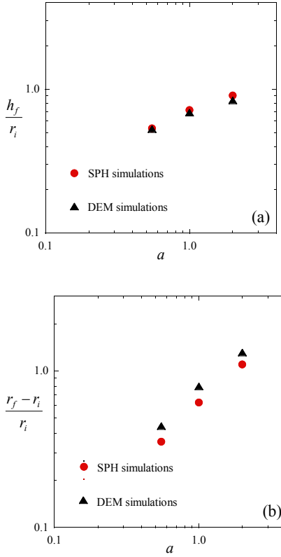
Figure 5. Comparison of SPH simulations, DEM simulations (a) normalized final height; (b)
