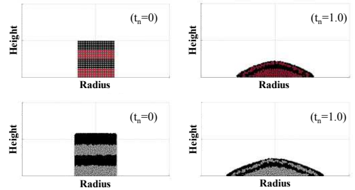
Figure 4. Initial column (at t_n = 0 ) and final deposit profile (at t_n = 1.0 ) for a column with a = 2.0 ; SPH (red/black) and DEM (gray/black)
