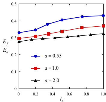
Figure 8. Normalized frictional energy dissipation \frac{E_f}{E_d} vs. t_n in DEM simulations
