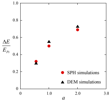
Figure 7. Normalized energy dissipation \frac{\Delta E}{E_{pi}} vs. a
