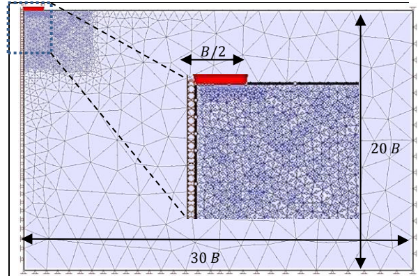
Figure 3: Boundary conditions, mesh and geometry details of the numerical model.
