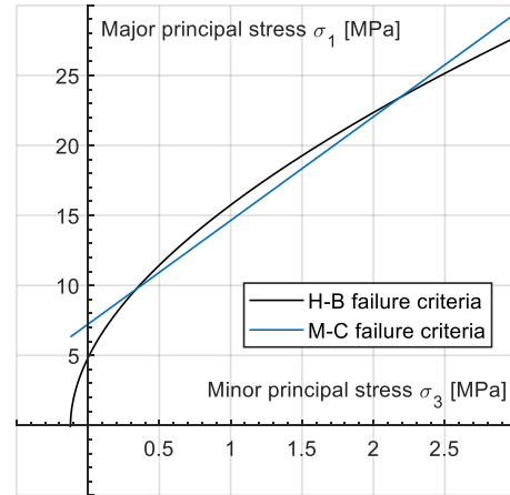
Figure 1: Mohr Coulomb and Hoek Brown failure envelope.
