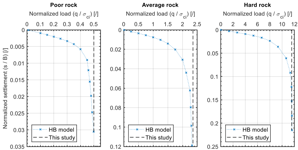
Figure 5: Load-displacement curves – Circular footing resting on poor, average and hard weightless rock
