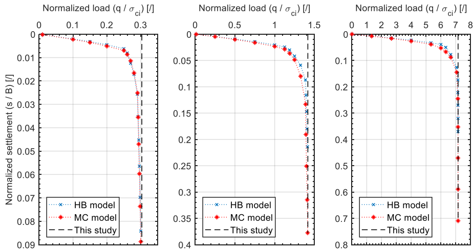
Figure 4: Load-displacement curves – Strip footing resting on poor, average and hard weightless rock.
