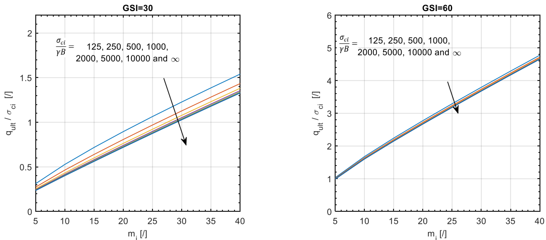
Figure 2: Normalized bearing capacity as a function of m_i for: (a) GSI=30 / (b) GSI=60
