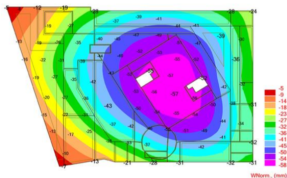
Figure 14. The settlement map of the foundation slab in ARSA model [mm]
