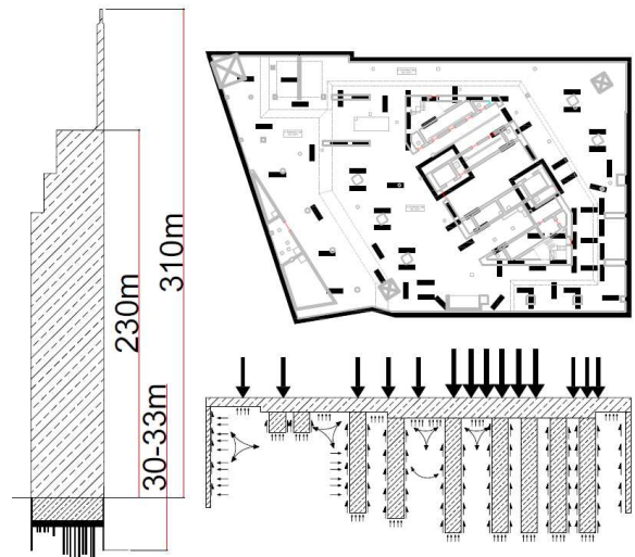
Figure 1. Geometry of the building, CPRF with the structures core and diagram of pile-soil-structure interaction
