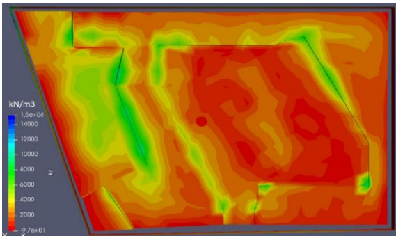
Figure 10. Ground stiffness under the foundation slab
