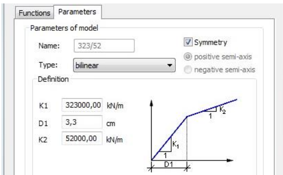
Figure 11. Support definition with nonlinear model in ARSA
