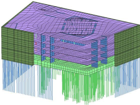
Figure 8. 3D view the underground part of the construction - diaphragm walls, slabs, cores, foundation slabs, barrettes
