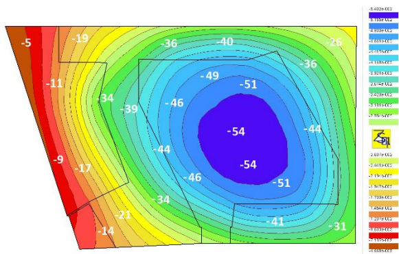
Figure 13. The settlement map of the foundation slab in ZSoil model [mm]
