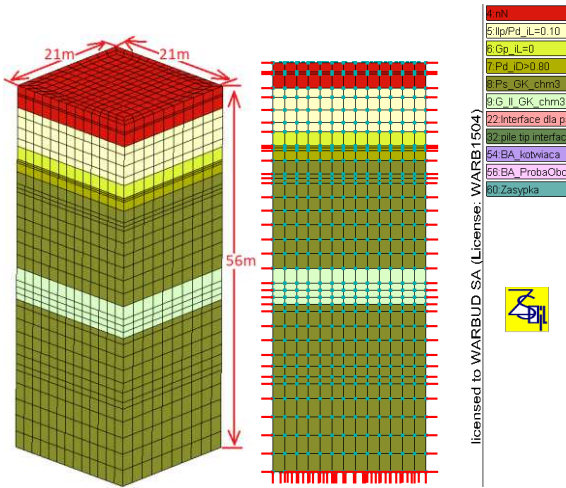
Figure 4. View of the 3D model of the barrette load testing
