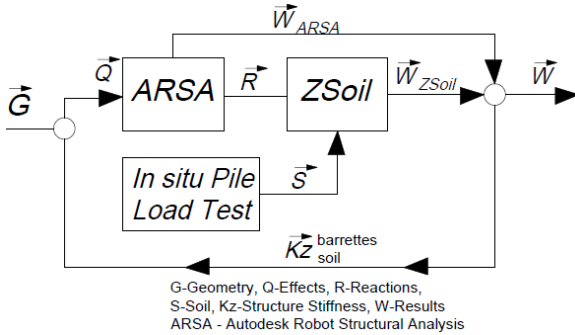
Figure 2. Simplified block diagram of the complex analysis
