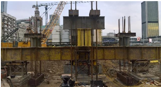
Figure 3. Structure of barrette load test - Barrette B82
