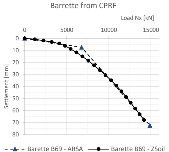
Figure 9. Load-settlement curve for barrette in CPRF in 3D ZSoil model with bilinear curve in ARSA model
