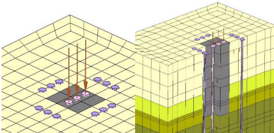
Figure 5. View of barrette B82 layout, anchor barrettes and the weakened soil layer in the ZSoil model
