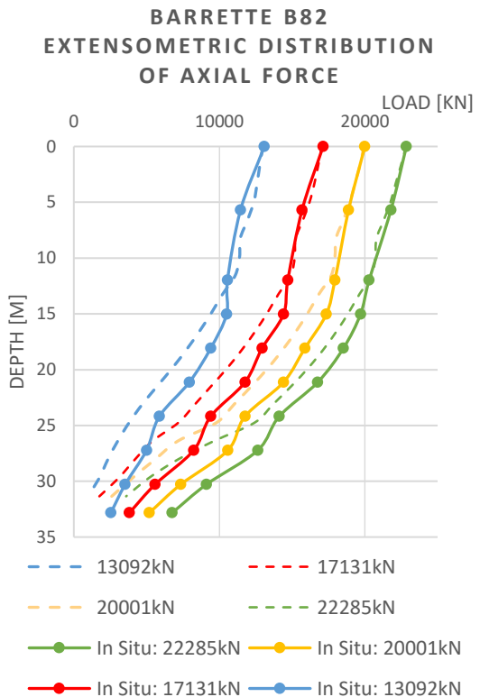
Figure 7. Distribution of axial force in barrette B82 from in situ test and ZSoil model
