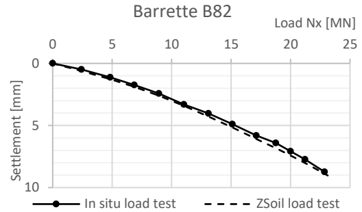
Figure 6. Load-settlement response of the head of the barrette under axial force from in-situ test and ZSoil model
