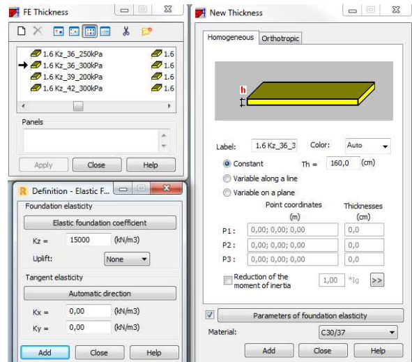
Figure 12. Definition of an elasticity modulus of the soil in ARSA
