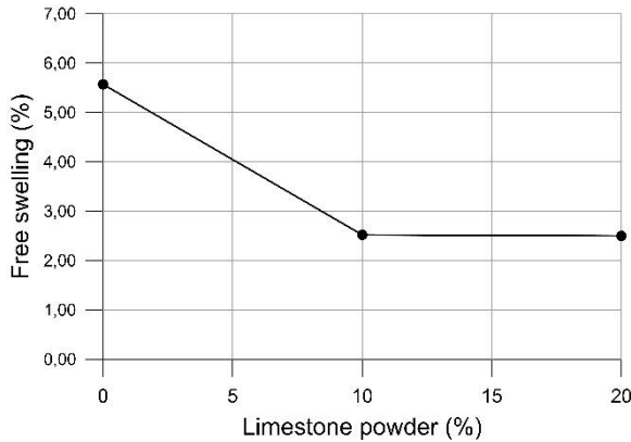
Figure 2. Free swell ratio values for soil with a different amount of limestone powder.
