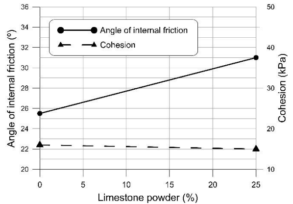
Figure 4. Variation of cohesion and angle of internal friction against percentage of limestone powder.
