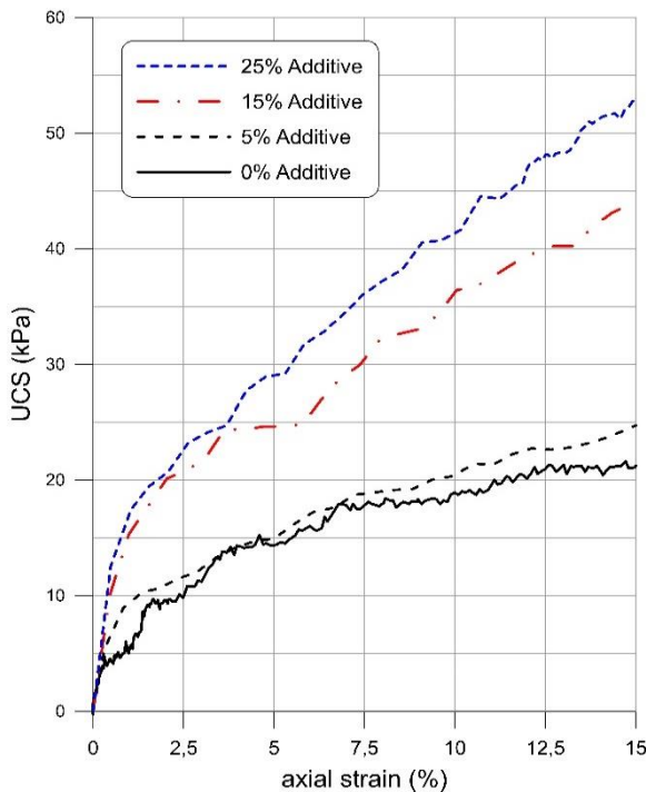
Figure 3. Unconfined compressive strengths for soil with a different amount of limestone powder.
