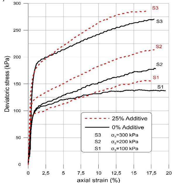
Figure 5. Strain vs. Stress for the three specimens of the samples with 0 and 25% of additive.
