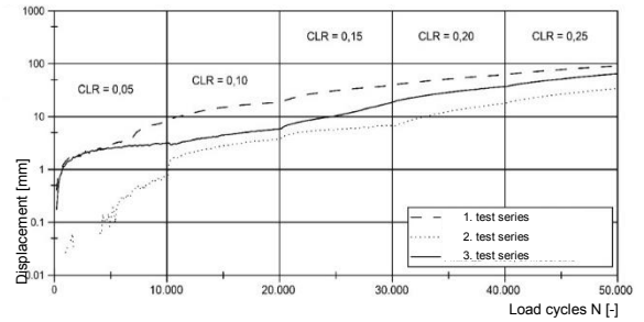
Figure 6. Accumulation of displacements over number of load cycles for different CLR and F_{min}/Q_u = 0.00
