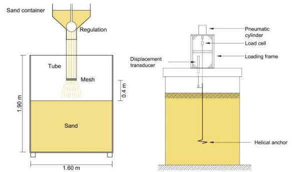
Figure 2. Experimental setup of tank with sand pluviation (left) and loading arrangement (right)
