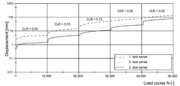
Figure 7. Accumulation of displacements over number of load cycles for different CLR and F_{min}/Q_u = 0.10
