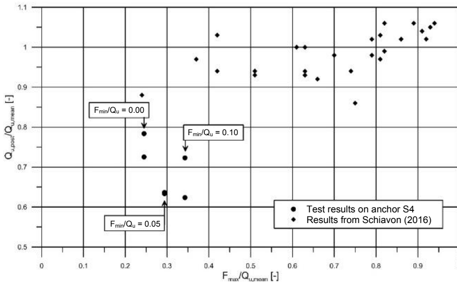
Figure 8. Comparison of the post-cyclic pullout capacity of anchor S4 with literature results
