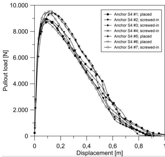
Figure 4. Load-displacement curves from monotonic pullout tests on anchor S4
