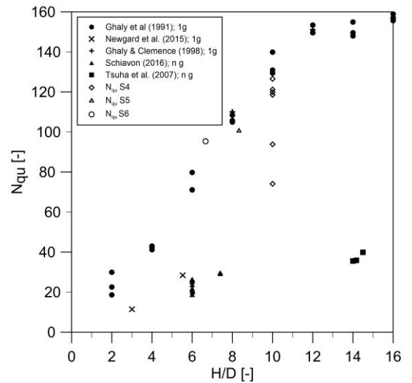
Figure 5. Comparison of measured pullout capacities with available test results
