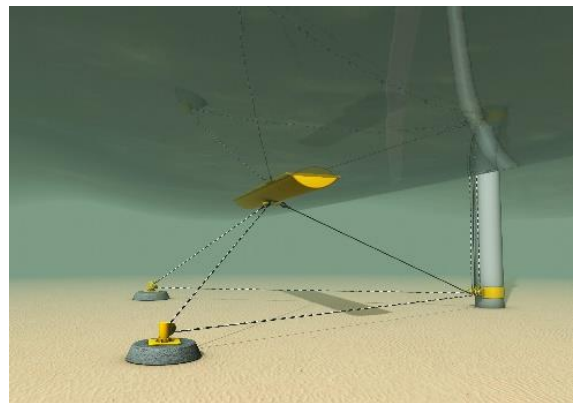
Figure 1. NEMOS wave energy converter (© NEMOS)
