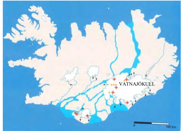
Figure 2. Areas affected by jökulhlaups attributed to volcanic activity in Iceland during the Holocene, shown in blue. Red crosses: volcanoes; yellow dots: geothermal spots; blue spots: glacial lagoons, arrows: directions of jökulhlaups (Björnsson, 2009).
