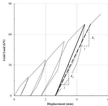
Figure 8. Definition of the footing stiffness during unloading and reloading
