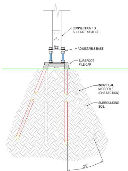
Figure 1. Installed footing in the ground (After Mehdizadeh et al., 2016)
