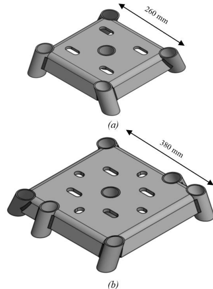
Figure 2. Top plate and piles configuration (a) S250 and (b) S400
