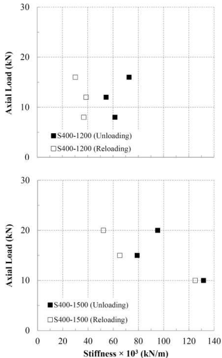
Figure 12. Variation of unloading/reloading stiffness with applied pullout load for S400
