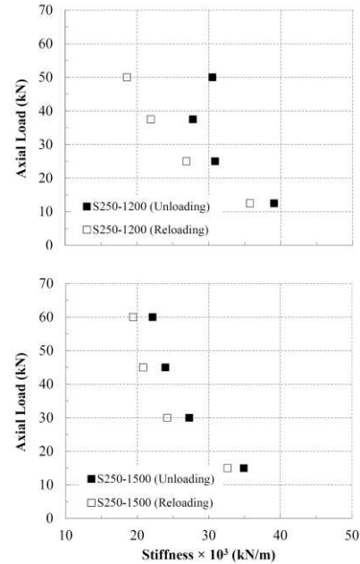
Figure 9. Variation of unloading/reloading stiffness with applied compressive load for S250
