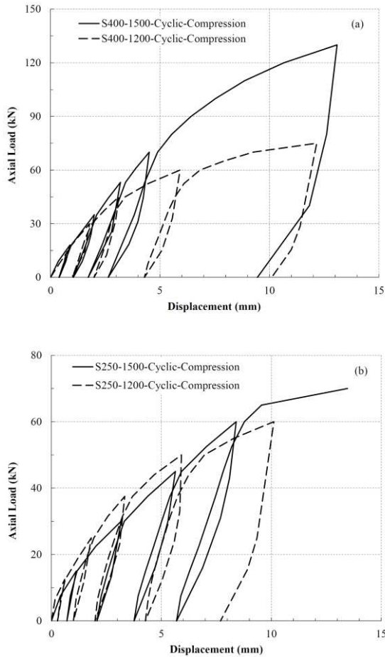
Figure 5. Load-settlement diagram for tested footings under cyclic compressive loadings (a) S400 and (b) S250 with 1200 and 1500 embedment depths
