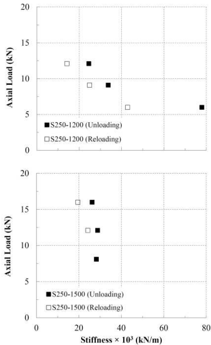
Figure 11. Variation of unloading/reloading stiffness with applied pullout load for S250
