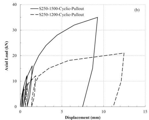
Figure 4. Load-settlement diagram for tested footings under cyclic pullout loadings (a) S400 and (b) S250 with 1200 and 1500 embedment depths
