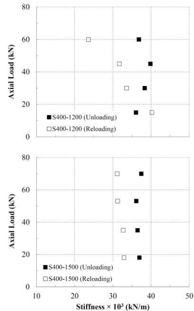
Figure 10. Variation of unloading/reloading stiffness with applied compressive load for S400
