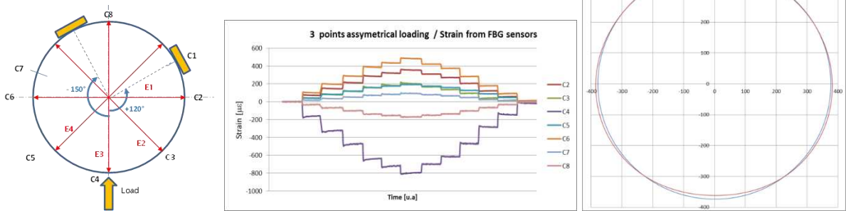
Figure 10: Case of asymmetrical 3-point loading: a) Positioning of FBG sensors and loading direction b) Response of FBG sensors and reversibility c) Elastic curve of structure under maximum loading calculated according to orthoradial strain values of FBG sensors.
