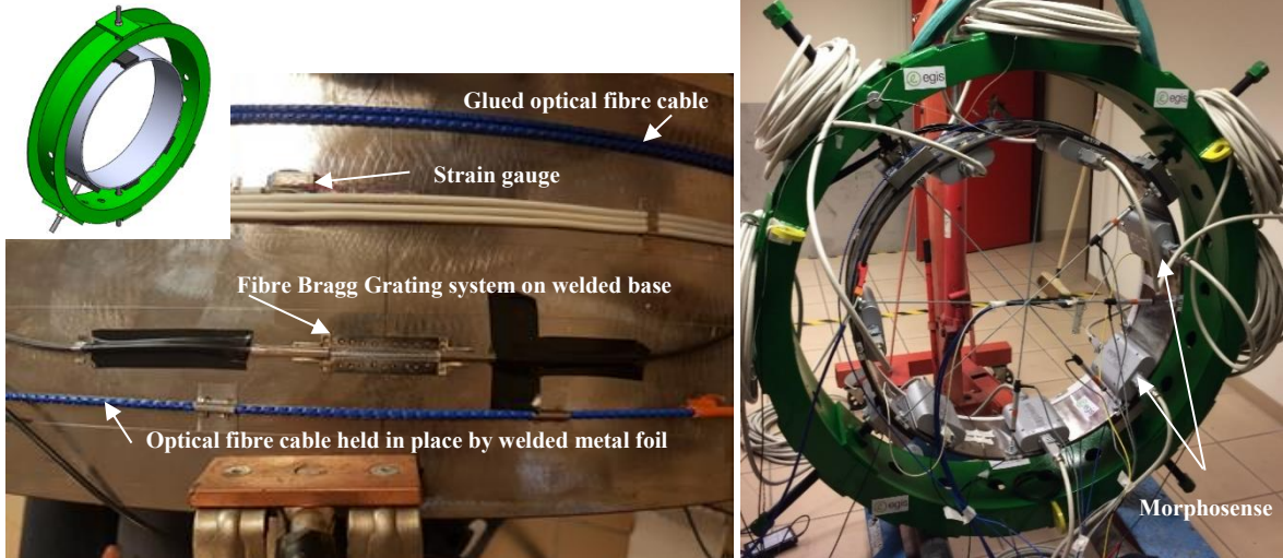
Figure 8: Photos of test bench and sensing equipment used
