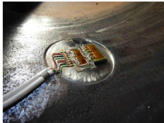
Figure 4 - Position of local strain measurements and photo of mounting
