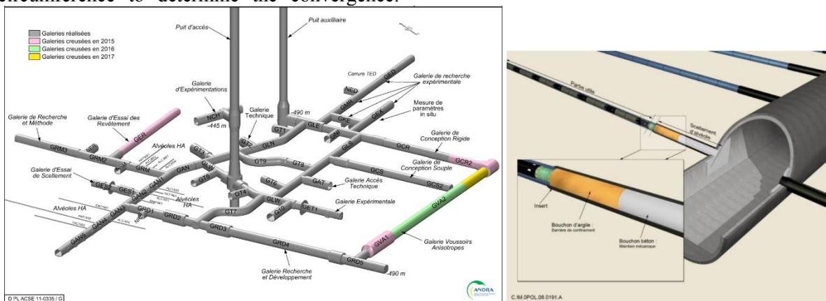
Figure 1. Layout of Andra underground laboratory galleries and diagram of an HL waste repository tunnel (2009 concept).
