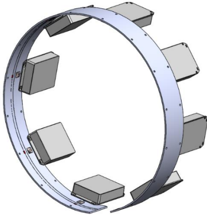
Figure 6 - Steel plate pre-equipped with Morphosense sensors and photo taken in micro-tunnel.
