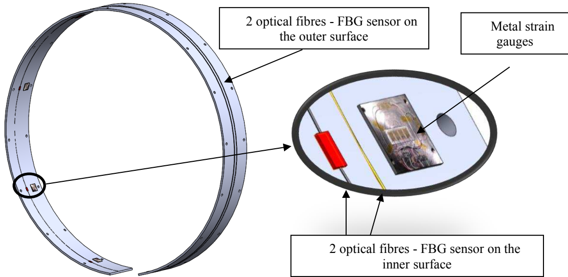
Figure 5 - Steel plate pre-equipped with optical fibres and strain gauges
