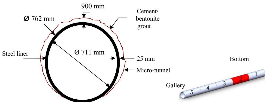
Figure 2 - Representation of a cross-section of the AHA1601 micro-tunnel and location of the liner equipped with sensors near the bottom (in red)
