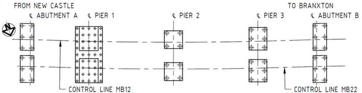
Figure 5. Layout plan of bridge foundations
