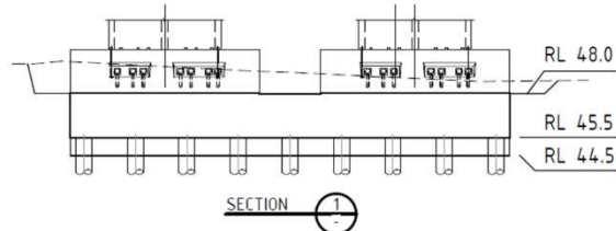
Figure 7. Piled raft plan and transverse cross-section
