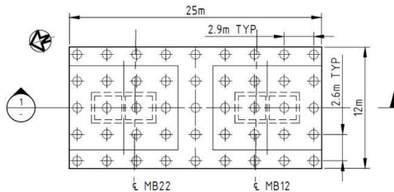
Figure 6. Layout plan of piled raft foundations
