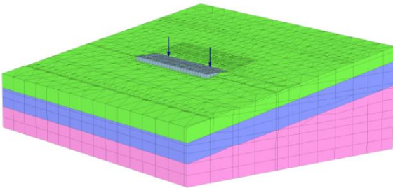
Figure 9. Piled raft Plaxis 3D model
