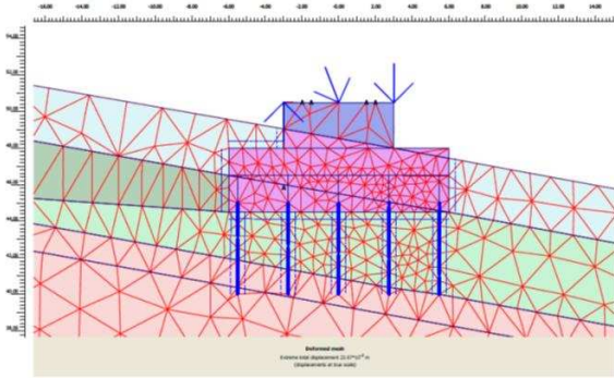
Figure 8. Piled raft Plaxis 2D model
