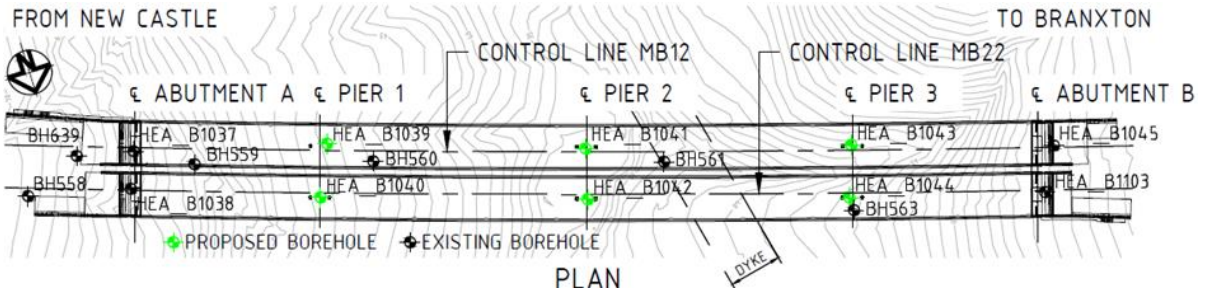
Figure 1. Plan of Bridge BW10 layout and proposed borehole locations
