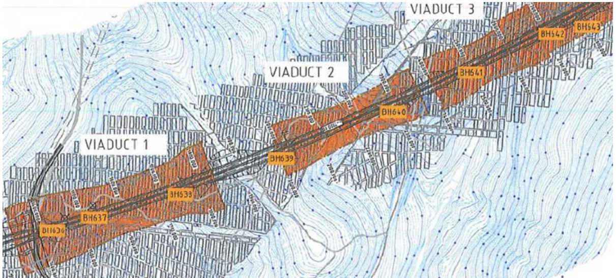
Figure 3. Extent of grouting and old mine working layout below bridges
