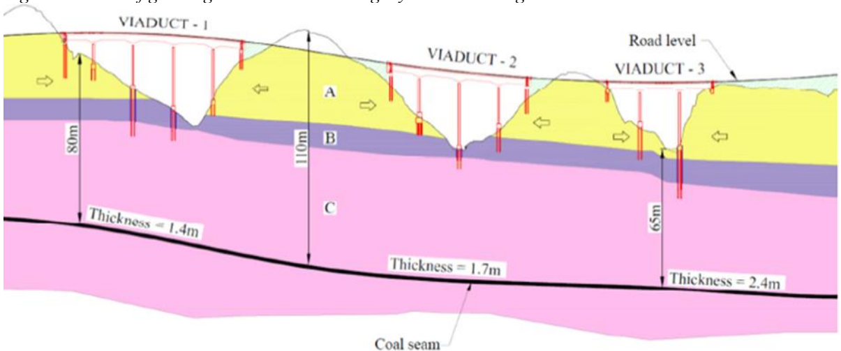
Figure 4. Elevation of proposed viaducts and depth to coal seam (after Pakharel et al).
