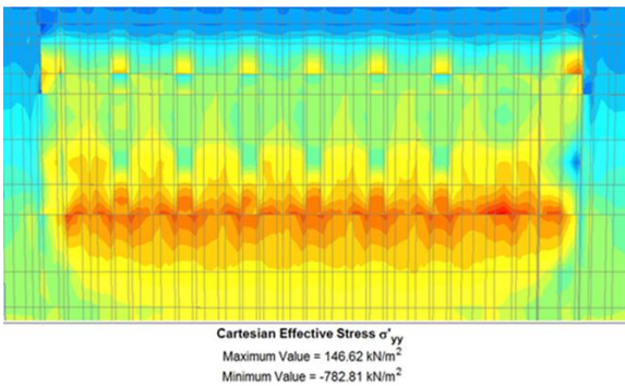
Figure 10. Vertical stress contour of piled raft
