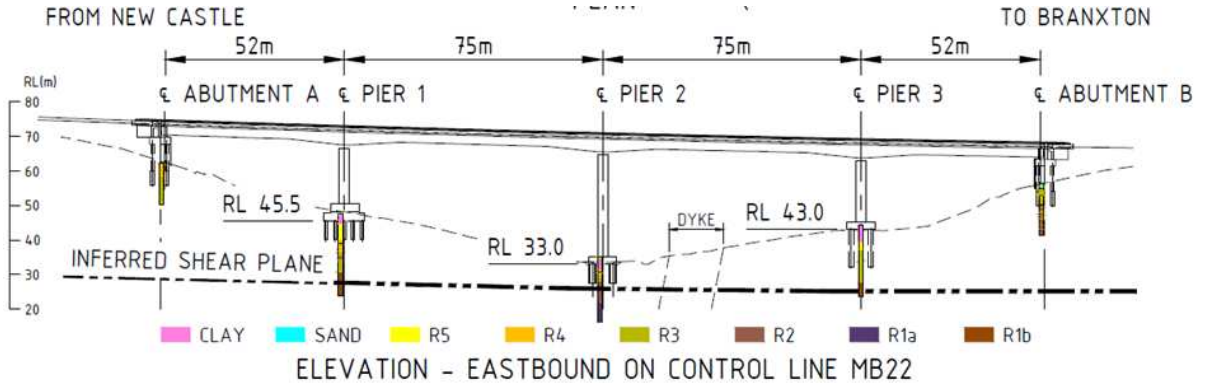
Figure 2. Geological cross-section with bridge shown
