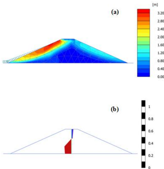
Figure 3. Model 1 under Kocaeli Earthquake, a) Total displacement distributions; b) Transmitted peak accelerations
