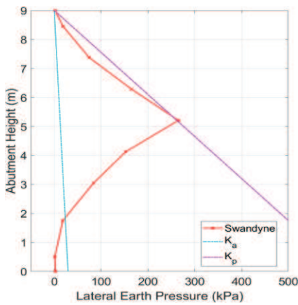
Fig. 4. Lateral earth pressure distribution after ratcheting cycles.
