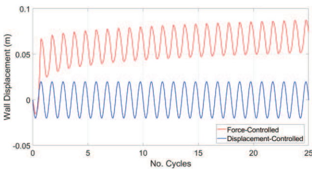
Fig. 5. Force and displacement-controlled comparison.
